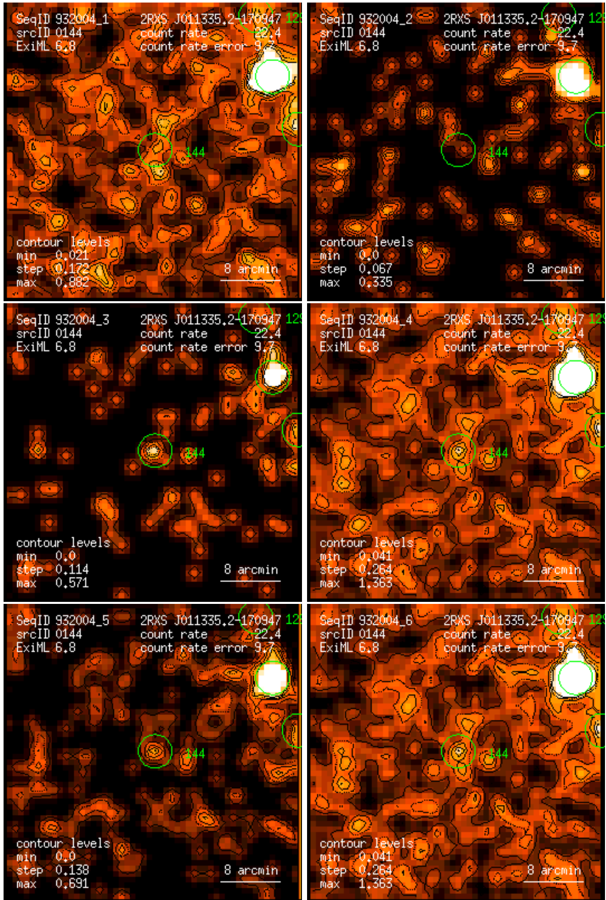
Figure 144: RASS 932004: detection 0144: band rate images, Gaussian filter: (1) PSPC channels 11 – 41, (2) 52 – 90, (3) 91 – 201, (4) 11 – 235, (5) 52 – 201, (6) 11 – 201. Broad band rates in counts/ks. Band rate contour levels in counts/ks/arcmin 2 .
