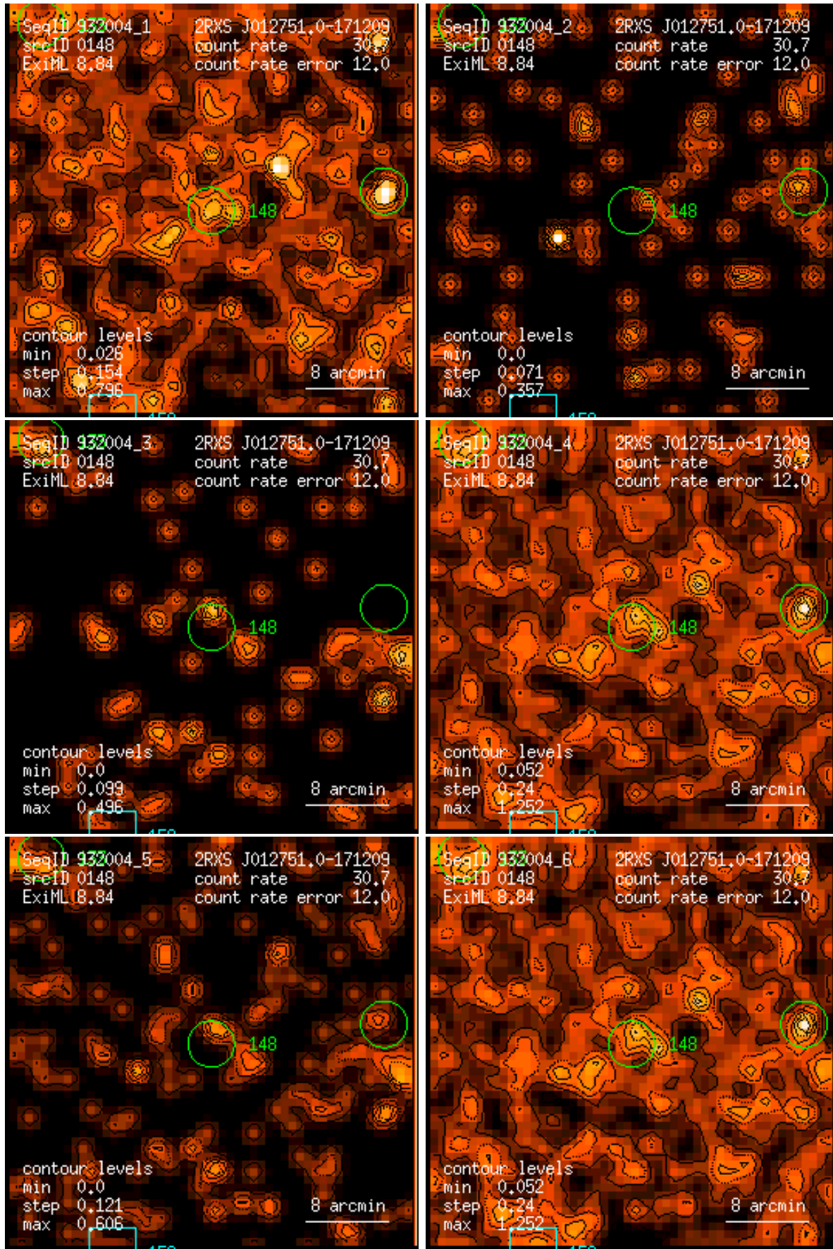
Figure 148: RASS 932004: detection 0148: band rate images, Gaussian filter: (1) PSPC channels 11 – 41, (2) 52 – 90, (3) 91 – 201, (4) 11 – 235, (5) 52 – 201, (6) 11 – 201. Broad band rates in counts/ks. Band rate contour levels in counts/ks/arcmin 2 .
