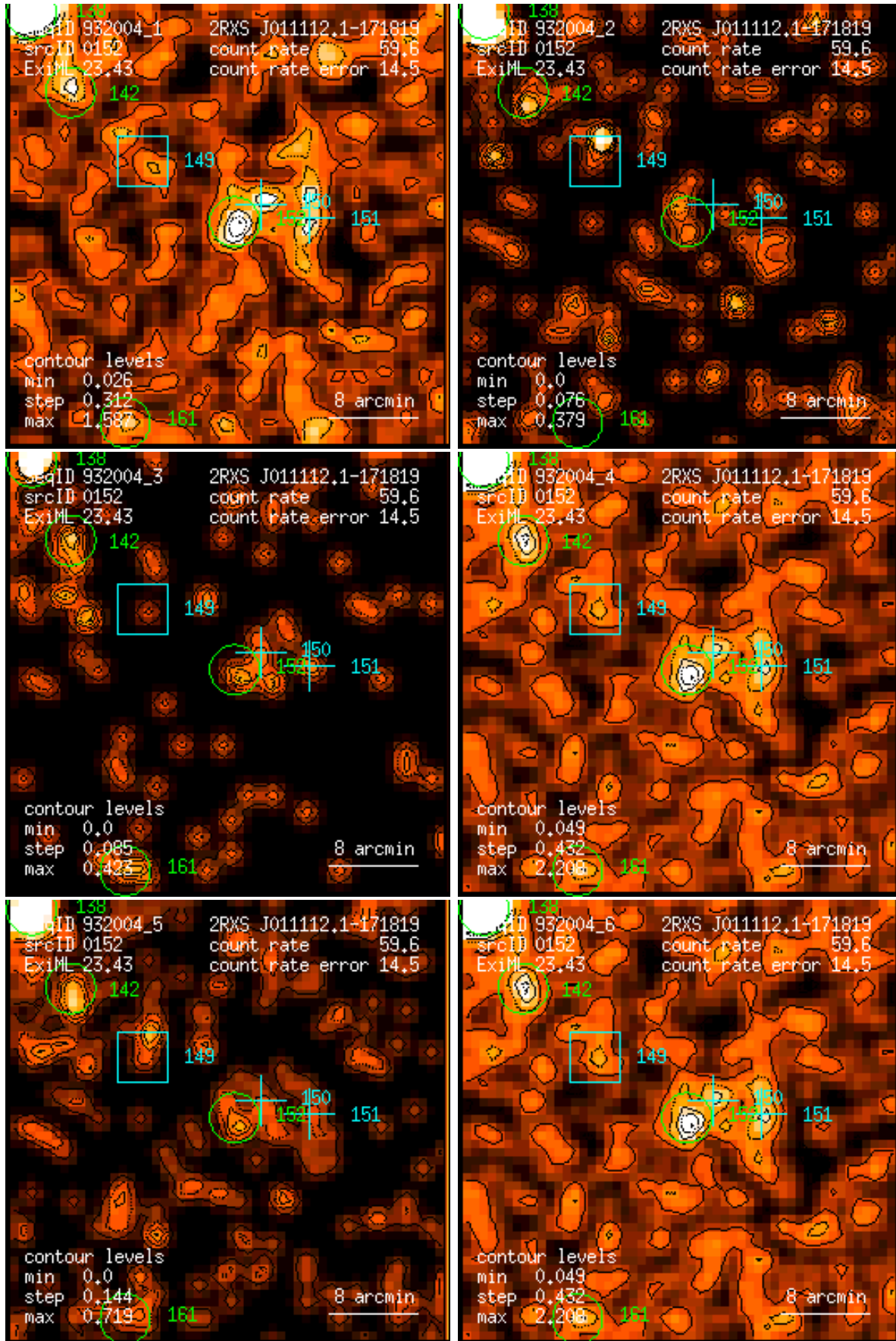
Figure 152: RASS 932004: detection 0152: band rate images, Gaussian filter: (1) PSPC channels 11 – 41, (2) 52 – 90, (3) 91 – 201, (4) 11 – 235, (5) 52 – 201, (6) 11 – 201. Broad band rates in counts/ks. Band rate contour levels in counts/ks/arcmin 2 .
