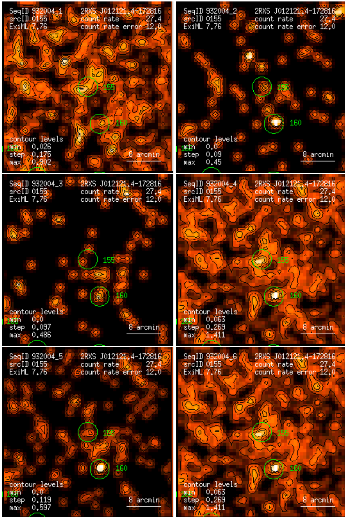
Figure 155: RASS 932004: detection 0155: band rate images, Gaussian filter: (1) PSPC channels 11 – 41, (2) 52 – 90, (3) 91 – 201, (4) 11 – 235, (5) 52 – 201, (6) 11 – 201. Broad band rates in counts/ks. Band rate contour levels in counts/ks/arcmin 2 .
