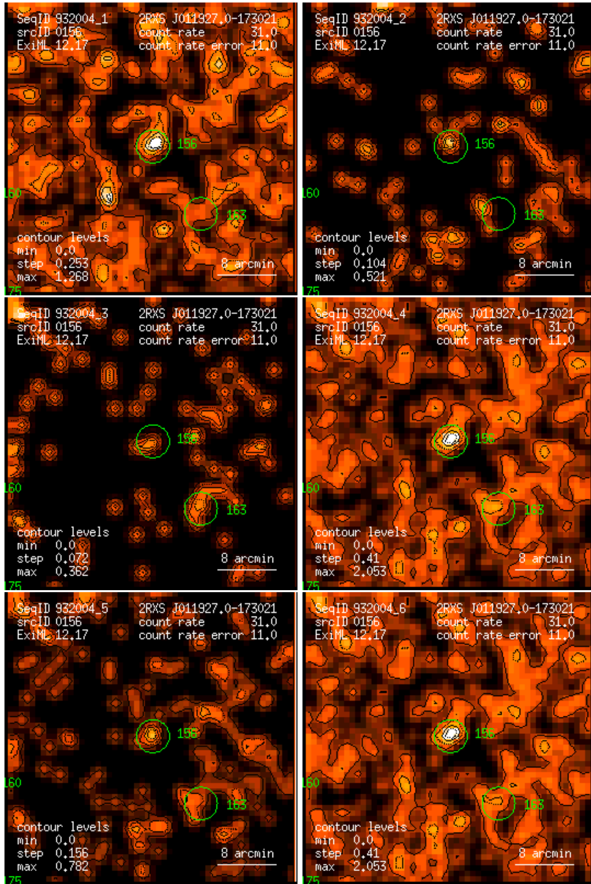
Figure 156: RASS 932004: detection 0156: band rate images, Gaussian filter: (1) PSPC channels 11 – 41, (2) 52 – 90, (3) 91 – 201, (4) 11 – 235, (5) 52 – 201, (6) 11 – 201. Broad band rates in counts/ks. Band rate contour levels in counts/ks/arcmin 2 .
