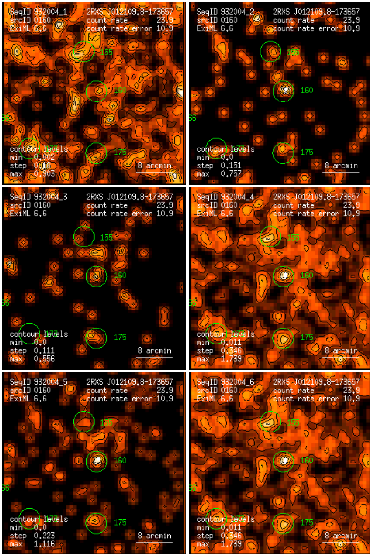
Figure 160: RASS 932004: detection 0160: band rate images, Gaussian filter: (1) PSPC channels 11 – 41, (2) 52 – 90, (3) 91 – 201, (4) 11 – 235, (5) 52 – 201, (6) 11 – 201. Broad band rates in counts/ks. Band rate contour levels in counts/ks/arcmin 2 .
