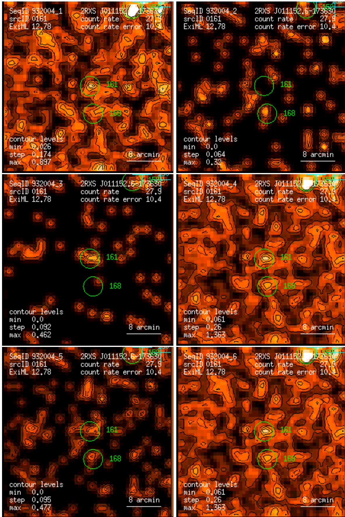
Figure 161: RASS 932004: detection 0161: band rate images, Gaussian filter: (1) PSPC channels 11 – 41, (2) 52 – 90, (3) 91 – 201, (4) 11 – 235, (5) 52 – 201, (6) 11 – 201. Broad band rates in counts/ks. Band rate contour levels in counts/ks/arcmin 2 .
