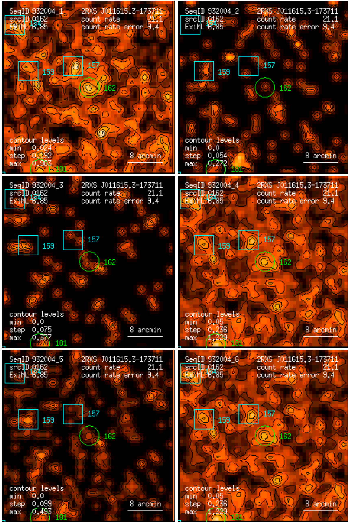
Figure 162: RASS 932004: detection 0162: band rate images, Gaussian filter: (1) PSPC channels 11 – 41, (2) 52 – 90, (3) 91 – 201, (4) 11 – 235, (5) 52 – 201, (6) 11 – 201. Broad band rates in counts/ks. Band rate contour levels in counts/ks/arcmin 2 .
