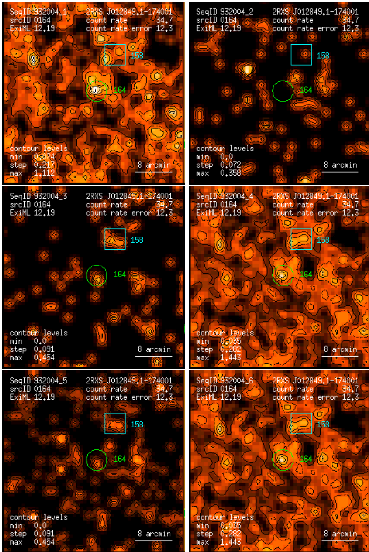
Figure 164: RASS 932004: detection 0164: band rate images, Gaussian filter: (1) PSPC channels 11 – 41, (2) 52 – 90, (3) 91 – 201, (4) 11 – 235, (5) 52 – 201, (6) 11 – 201. Broad band rates in counts/ks. Band rate contour levels in counts/ks/arcmin 2 .
