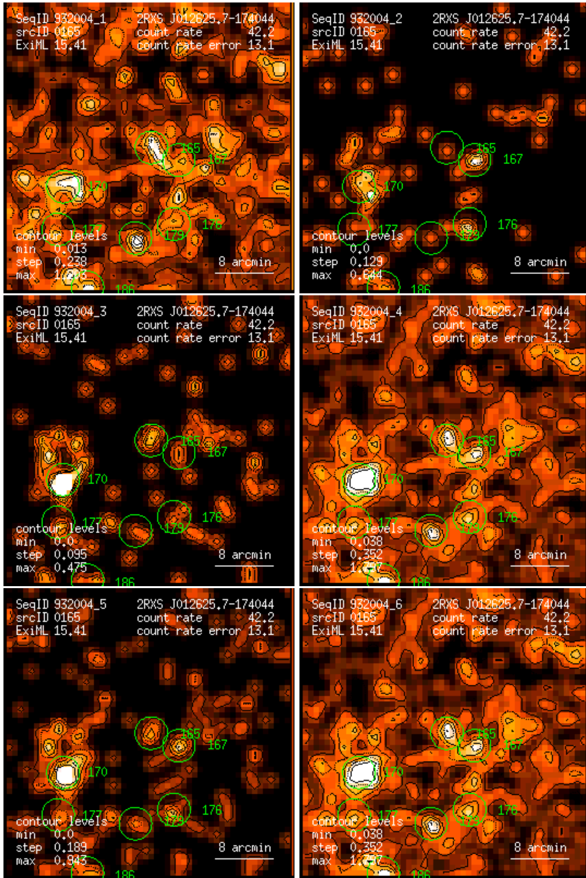
Figure 165: RASS 932004: detection 0165: band rate images, Gaussian filter: (1) PSPC channels 11 – 41, (2) 52 – 90, (3) 91 – 201, (4) 11 – 235, (5) 52 – 201, (6) 11 – 201. Broad band rates in counts/ks. Band rate contour levels in counts/ks/arcmin 2 .
