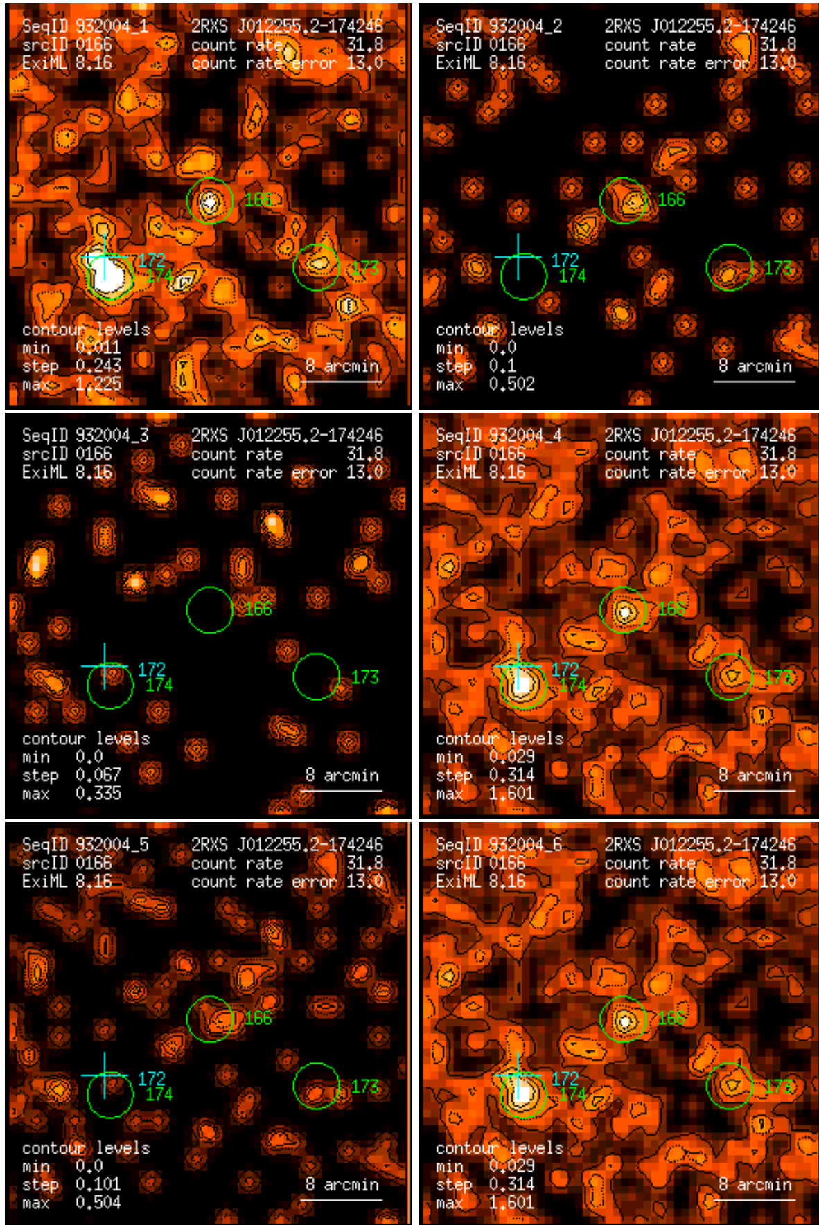
Figure 166: RASS 932004: detection 0166: band rate images, Gaussian filter: (1) PSPC channels 11 – 41, (2) 52 – 90, (3) 91 – 201, (4) 11 – 235, (5) 52 – 201, (6) 11 – 201. Broad band rates in counts/ks. Band rate contour levels in counts/ks/arcmin 2 .
