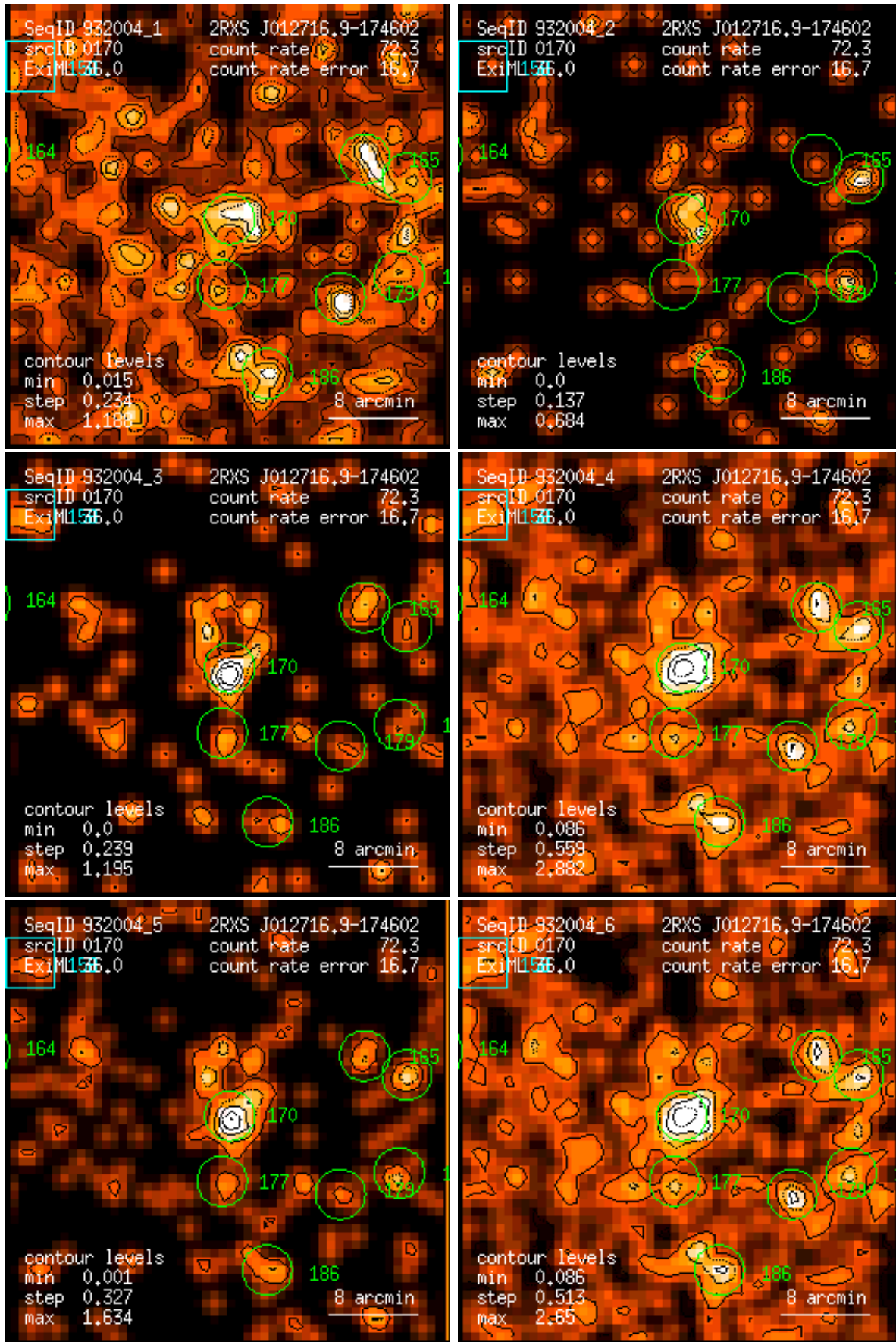
Figure 170: RASS 932004: detection 0170: band rate images, Gaussian filter: (1) PSPC channels 11 – 41, (2) 52 – 90, (3) 91 – 201, (4) 11 – 235, (5) 52 – 201, (6) 11 – 201. Broad band rates in counts/ks. Band rate contour levels in counts/ks/arcmin 2 .
