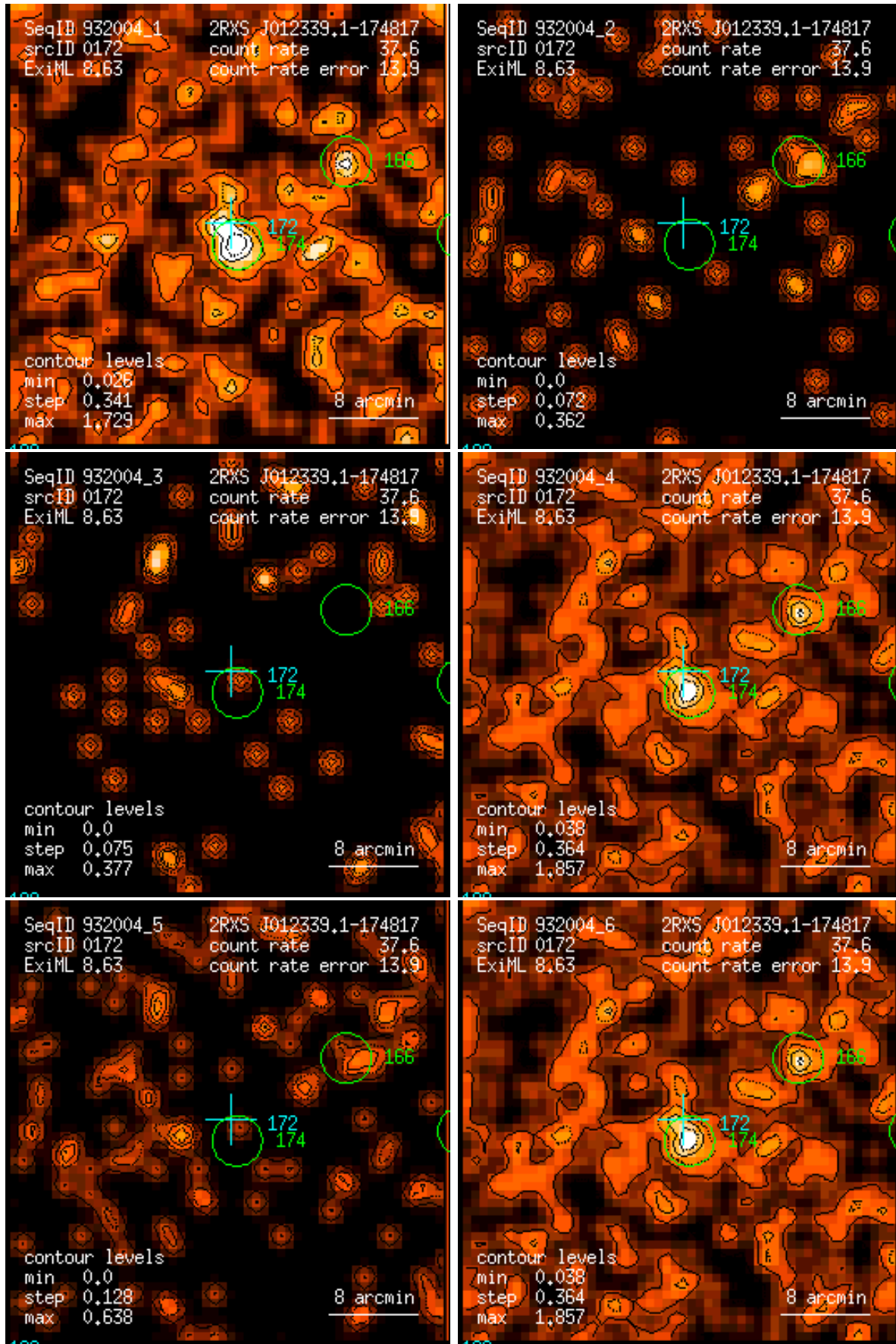
Figure 172: RASS 932004: detection 0172: band rate images, Gaussian filter: (1) PSPC channels 11 – 41, (2) 52 – 90, (3) 91 – 201, (4) 11 – 235, (5) 52 – 201, (6) 11 – 201. Broad band rates in counts/ks. Band rate contour levels in counts/ks/arcmin 2 .
