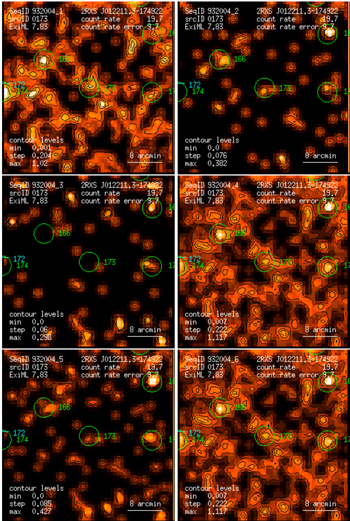
Figure 173: RASS 932004: detection 0173: band rate images, Gaussian filter: (1) PSPC channels 11 – 41, (2) 52 – 90, (3) 91 – 201, (4) 11 – 235, (5) 52 – 201, (6) 11 – 201. Broad band rates in counts/ks. Band rate contour levels in counts/ks/arcmin 2 .
