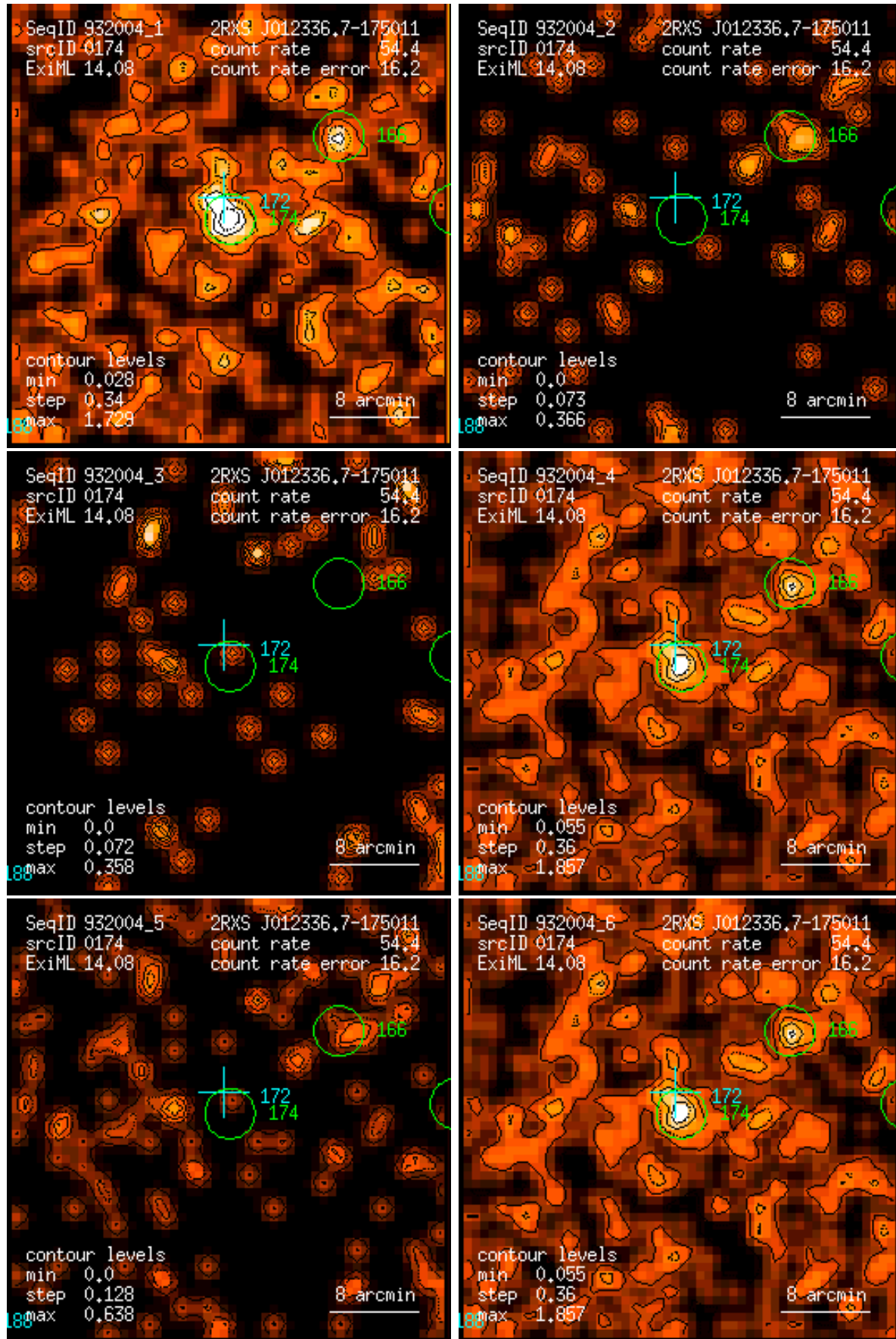
Figure 174: RASS 932004: detection 0174: band rate images, Gaussian filter: (1) PSPC channels 11 – 41, (2) 52 – 90, (3) 91 – 201, (4) 11 – 235, (5) 52 – 201, (6) 11 – 201. Broad band rates in counts/ks. Band rate contour levels in counts/ks/arcmin 2 .
