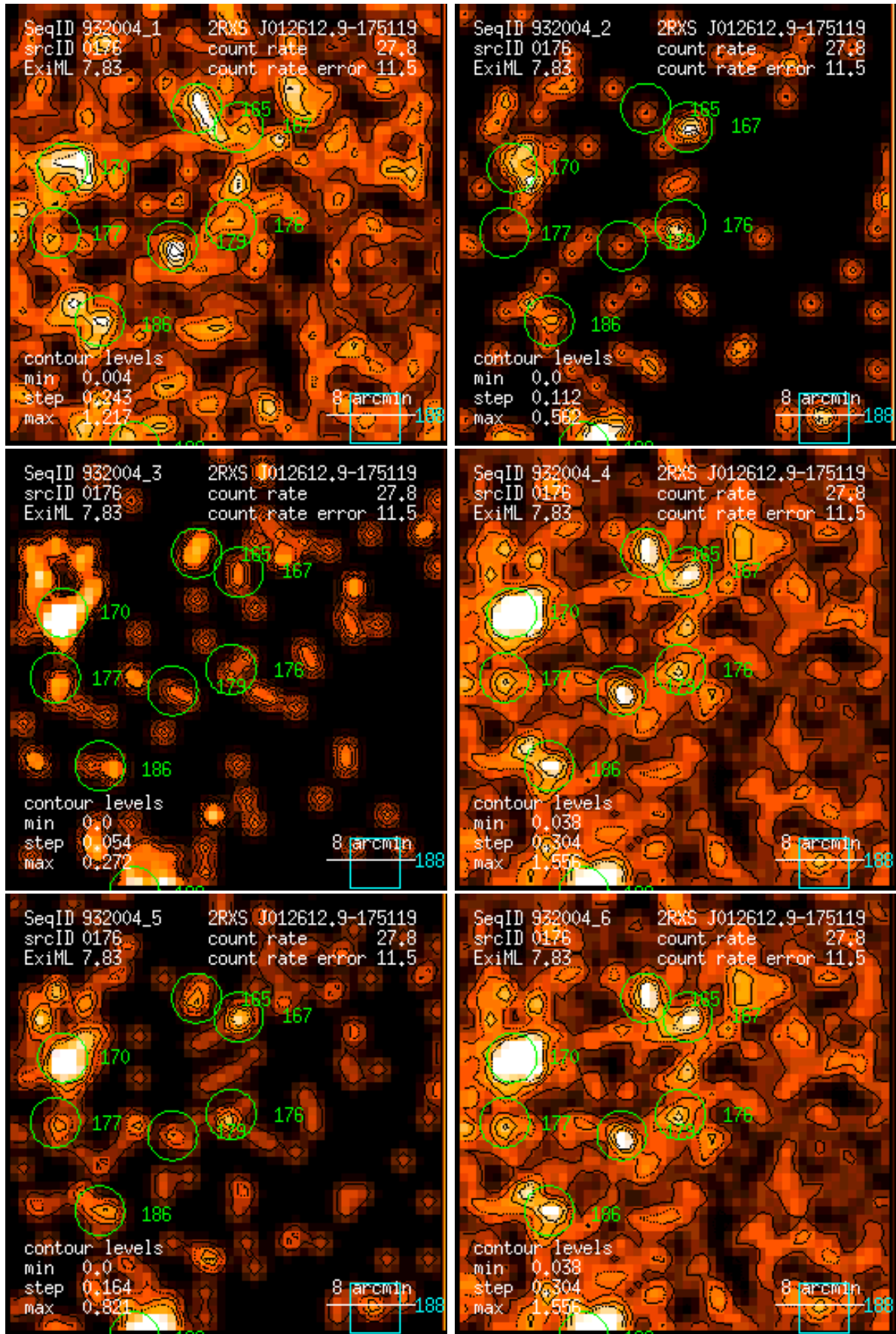
Figure 176: RASS 932004: detection 0176: band rate images, Gaussian filter: (1) PSPC channels 11 – 41, (2) 52 – 90, (3) 91 – 201, (4) 11 – 235, (5) 52 – 201, (6) 11 – 201. Broad band rates in counts/ks. Band rate contour levels in counts/ks/arcmin 2 .
