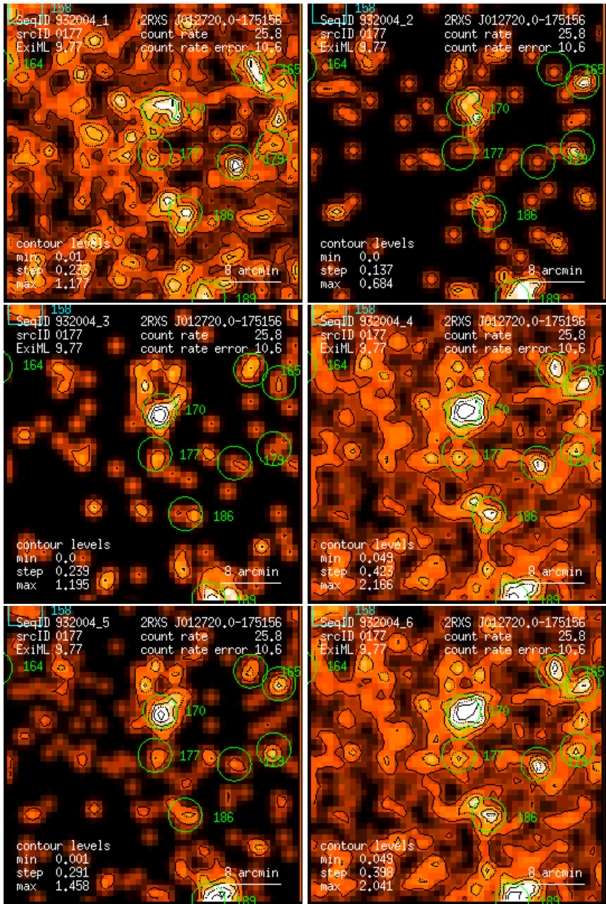
Figure 177: RASS 932004: detection 0177: band rate images, Gaussian filter: (1) PSPC channels 11 – 41, (2) 52 – 90, (3) 91 – 201, (4) 11 – 235, (5) 52 – 201, (6) 11 – 201. Broad band rates in counts/ks. Band rate contour levels in counts/ks/arcmin 2 .
