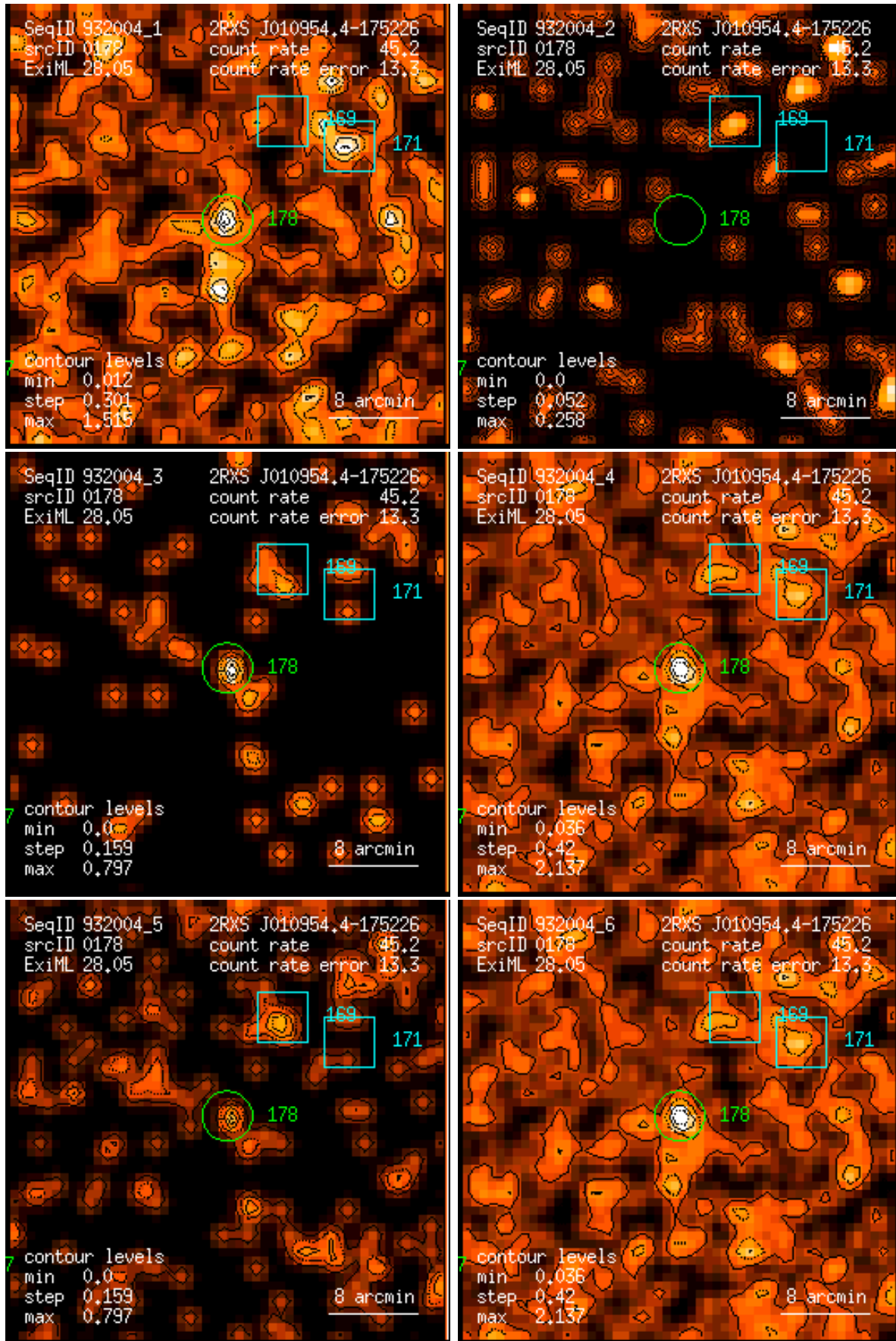
Figure 178: RASS 932004: detection 0178: band rate images, Gaussian filter: (1) PSPC channels 11 – 41, (2) 52 – 90, (3) 91 – 201, (4) 11 – 235, (5) 52 – 201, (6) 11 – 201. Broad band rates in counts/ks. Band rate contour levels in counts/ks/arcmin 2 .
