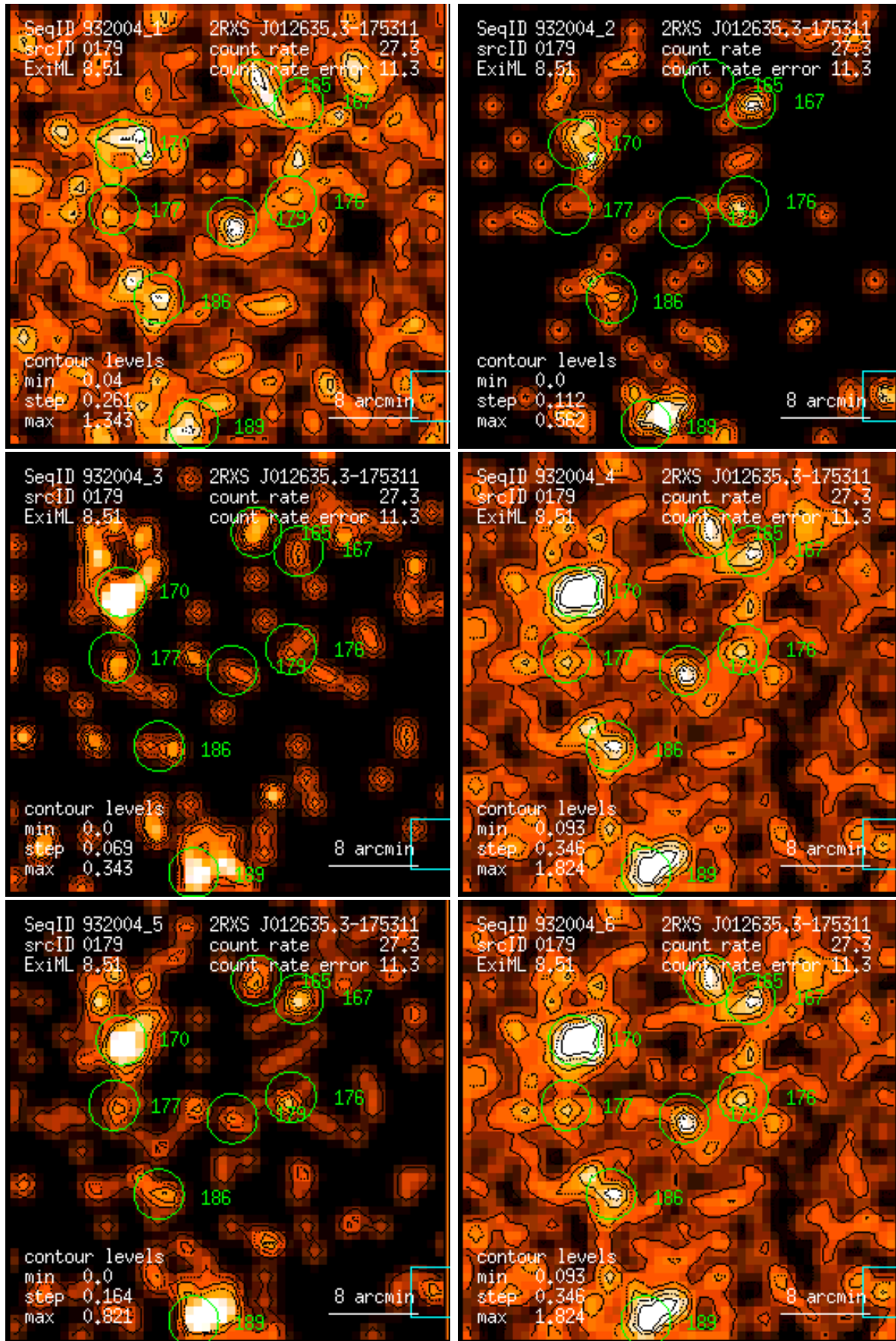
Figure 179: RASS 932004: detection 0179: band rate images, Gaussian filter: (1) PSPC channels 11 – 41, (2) 52 – 90, (3) 91 – 201, (4) 11 – 235, (5) 52 – 201, (6) 11 – 201. Broad band rates in counts/ks. Band rate contour levels in counts/ks/arcmin 2 .
