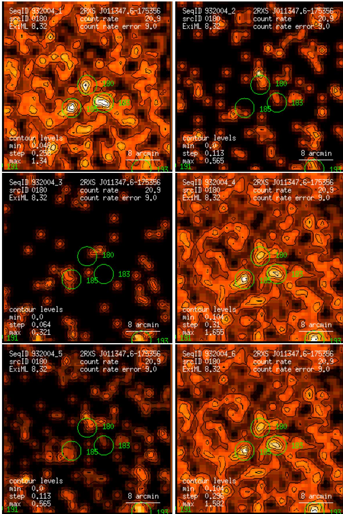
Figure 180: RASS 932004: detection 0180: band rate images, Gaussian filter: (1) PSPC channels 11 – 41, (2) 52 – 90, (3) 91 – 201, (4) 11 – 235, (5) 52 – 201, (6) 11 – 201. Broad band rates in counts/ks. Band rate contour levels in counts/ks/arcmin 2 .
