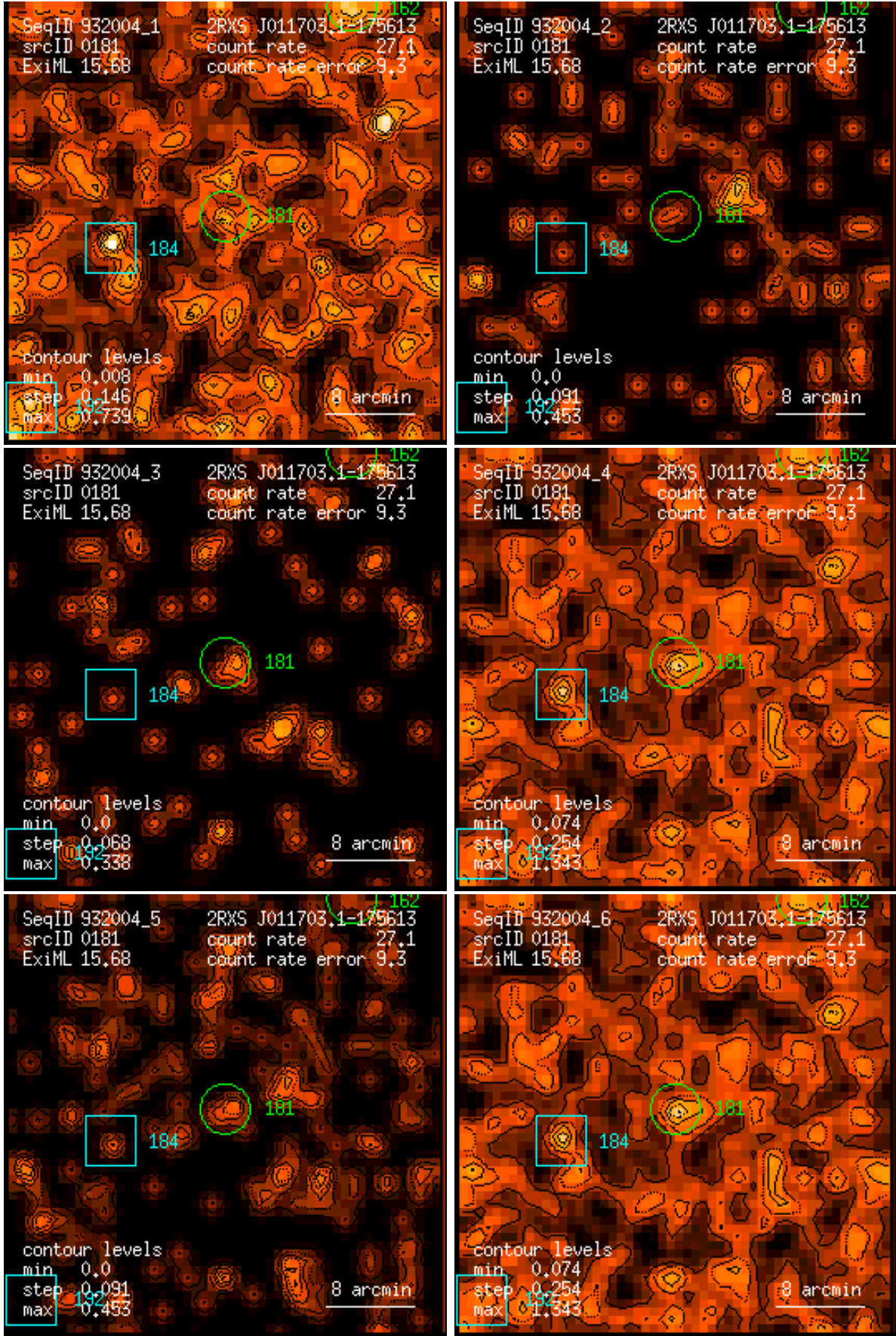
Figure 181: RASS 932004: detection 0181: band rate images, Gaussian filter: (1) PSPC channels 11 – 41, (2) 52 – 90, (3) 91 – 201, (4) 11 – 235, (5) 52 – 201, (6) 11 – 201. Broad band rates in counts/ks. Band rate contour levels in counts/ks/arcmin 2 .
