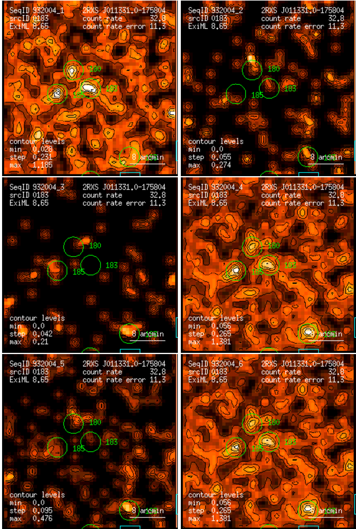
Figure 183: RASS 932004: detection 0183: band rate images, Gaussian filter: (1) PSPC channels 11 – 41, (2) 52 – 90, (3) 91 – 201, (4) 11 – 235, (5) 52 – 201, (6) 11 – 201. Broad band rates in counts/ks. Band rate contour levels in counts/ks/arcmin 2 .
