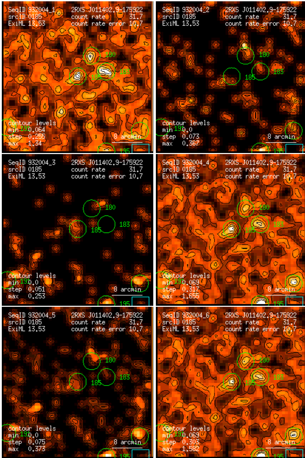
Figure 185: RASS 932004: detection 0185: band rate images, Gaussian filter: (1) PSPC channels 11 – 41, (2) 52 – 90, (3) 91 – 201, (4) 11 – 235, (5) 52 – 201, (6) 11 – 201. Broad band rates in counts/ks. Band rate contour levels in counts/ks/arcmin 2 .
