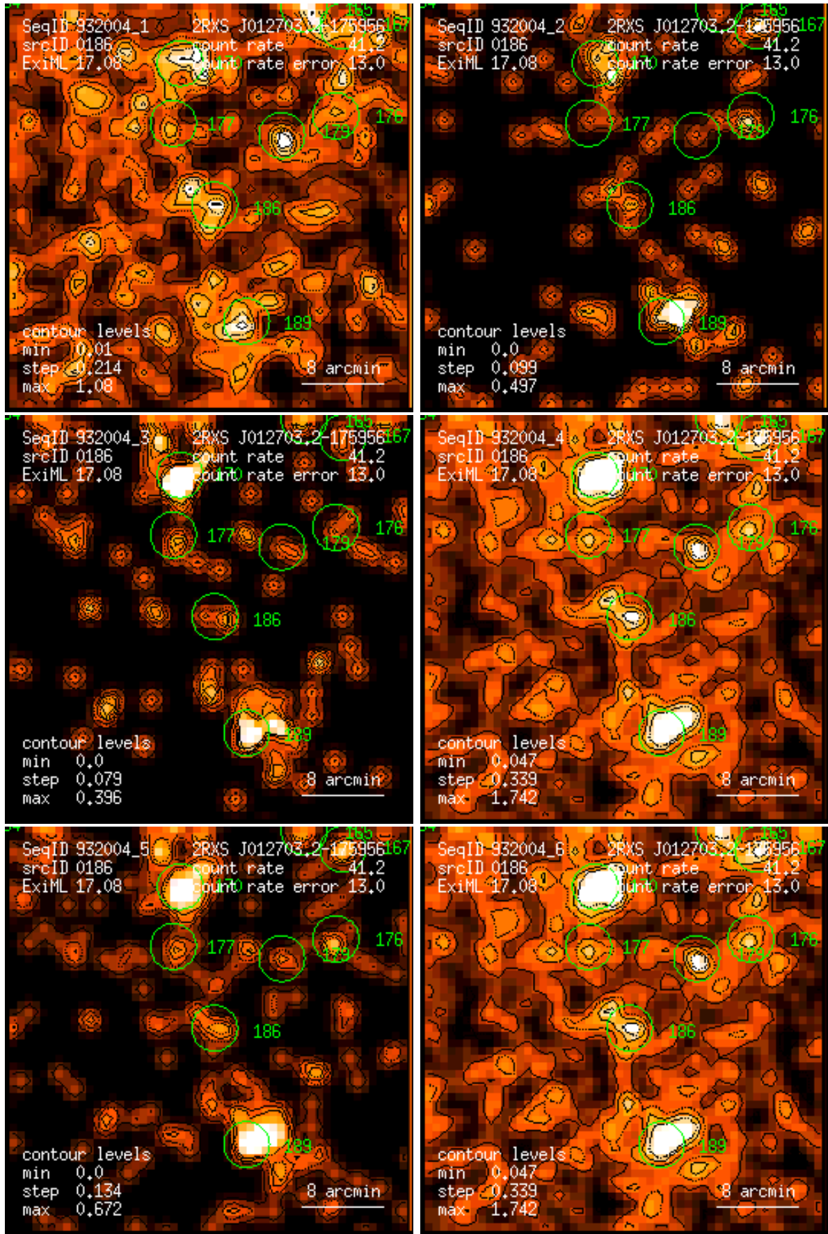
Figure 186: RASS 932004: detection 0186: band rate images, Gaussian filter: (1) PSPC channels 11 – 41, (2) 52 – 90, (3) 91 – 201, (4) 11 – 235, (5) 52 – 201, (6) 11 – 201. Broad band rates in counts/ks. Band rate contour levels in counts/ks/arcmin 2 .
