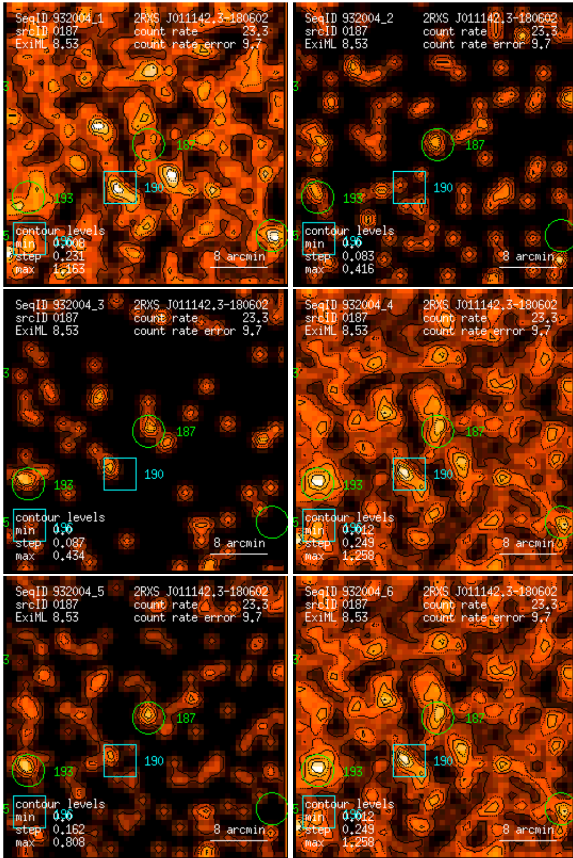
Figure 187: RASS 932004: detection 0187: band rate images, Gaussian filter: (1) PSPC channels 11 – 41, (2) 52 – 90, (3) 91 – 201, (4) 11 – 235, (5) 52 – 201, (6) 11 – 201. Broad band rates in counts/ks. Band rate contour levels in counts/ks/arcmin 2 .
