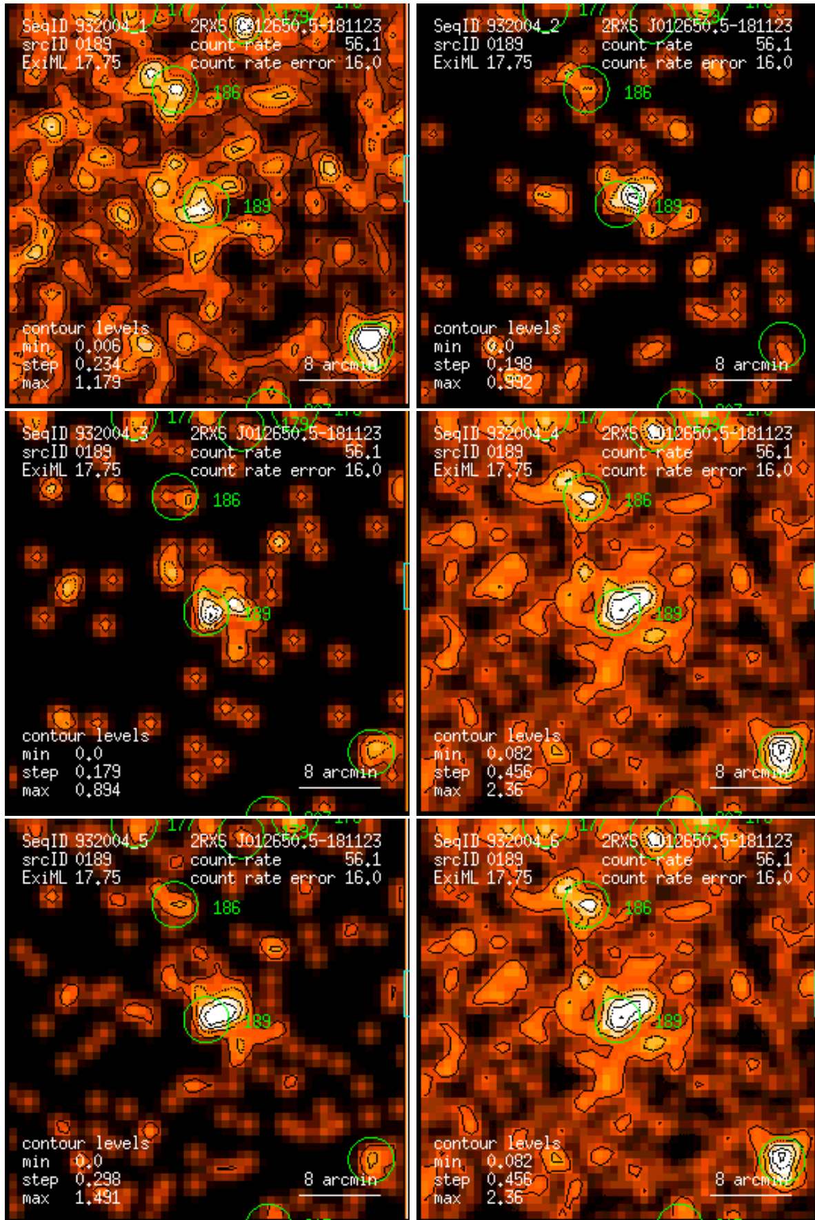
Figure 189: RASS 932004: detection 0189: band rate images, Gaussian filter: (1) PSPC channels 11 – 41, (2) 52 – 90, (3) 91 – 201, (4) 11 – 235, (5) 52 – 201, (6) 11 – 201. Broad band rates in counts/ks. Band rate contour levels in counts/ks/arcmin 2 .
