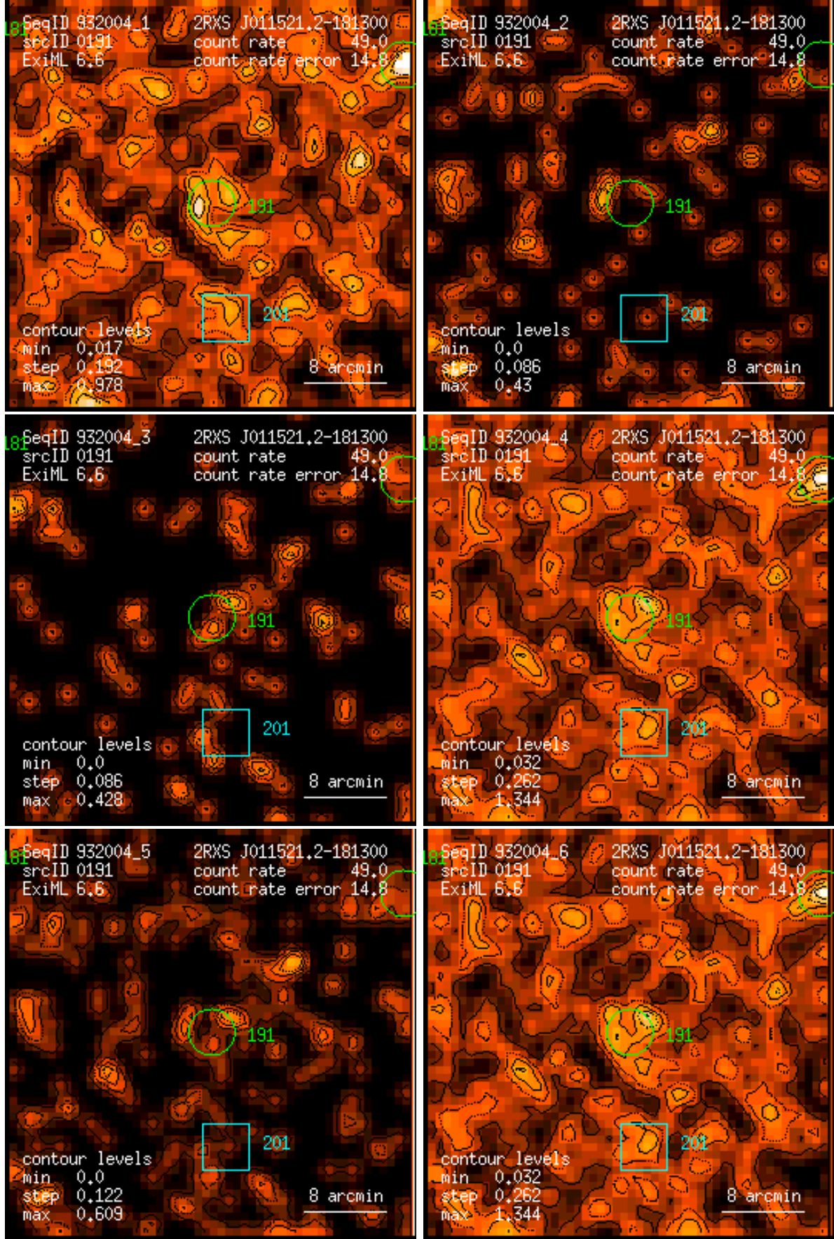
Figure 191: RASS 932004: detection 0191: band rate images, Gaussian filter: (1) PSPC channels 11 – 41, (2) 52 – 90, (3) 91 – 201, (4) 11 – 235, (5) 52 – 201, (6) 11 – 201. Broad band rates in counts/ks. Band rate contour levels in counts/ks/arcmin 2 .
