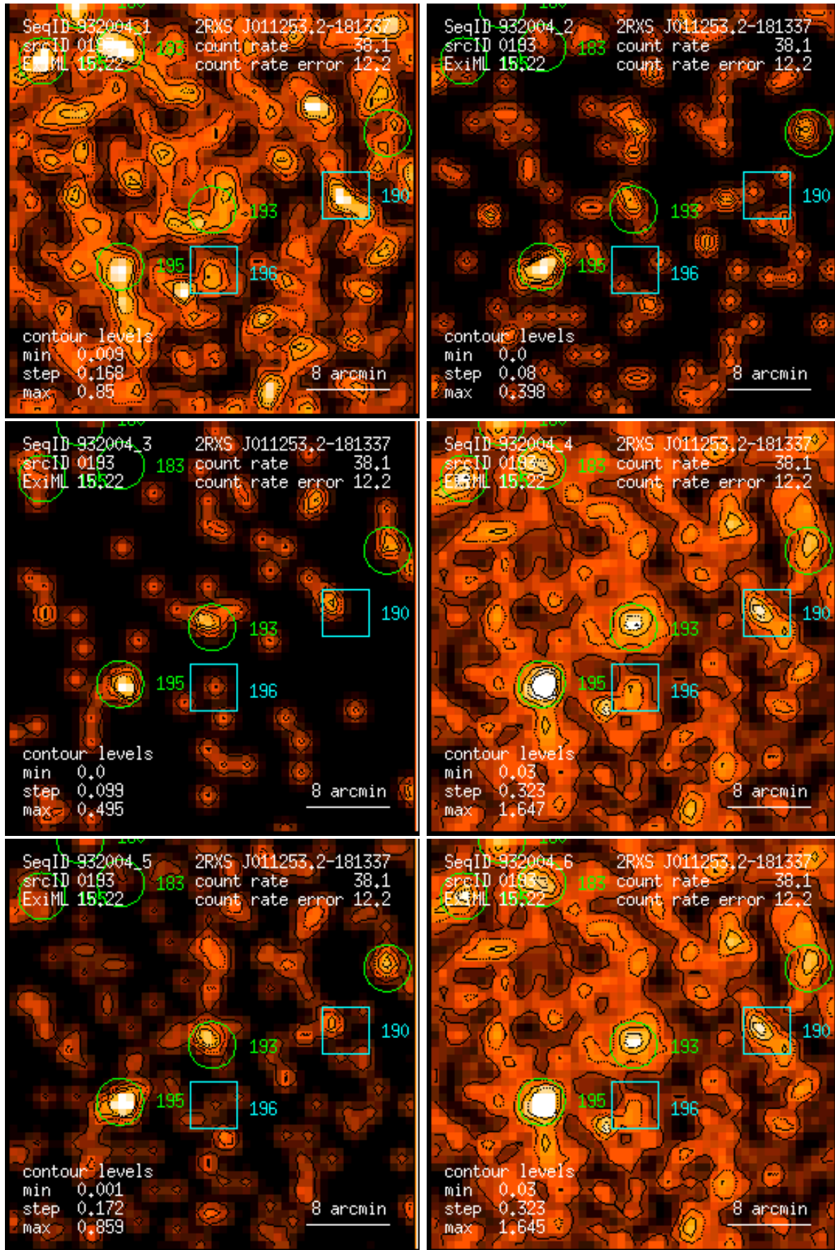
Figure 193: RASS 932004: detection 0193: band rate images, Gaussian filter: (1) PSPC channels 11 – 41, (2) 52 – 90, (3) 91 – 201, (4) 11 – 235, (5) 52 – 201, (6) 11 – 201. Broad band rates in counts/ks. Band rate contour levels in counts/ks/arcmin 2 .
