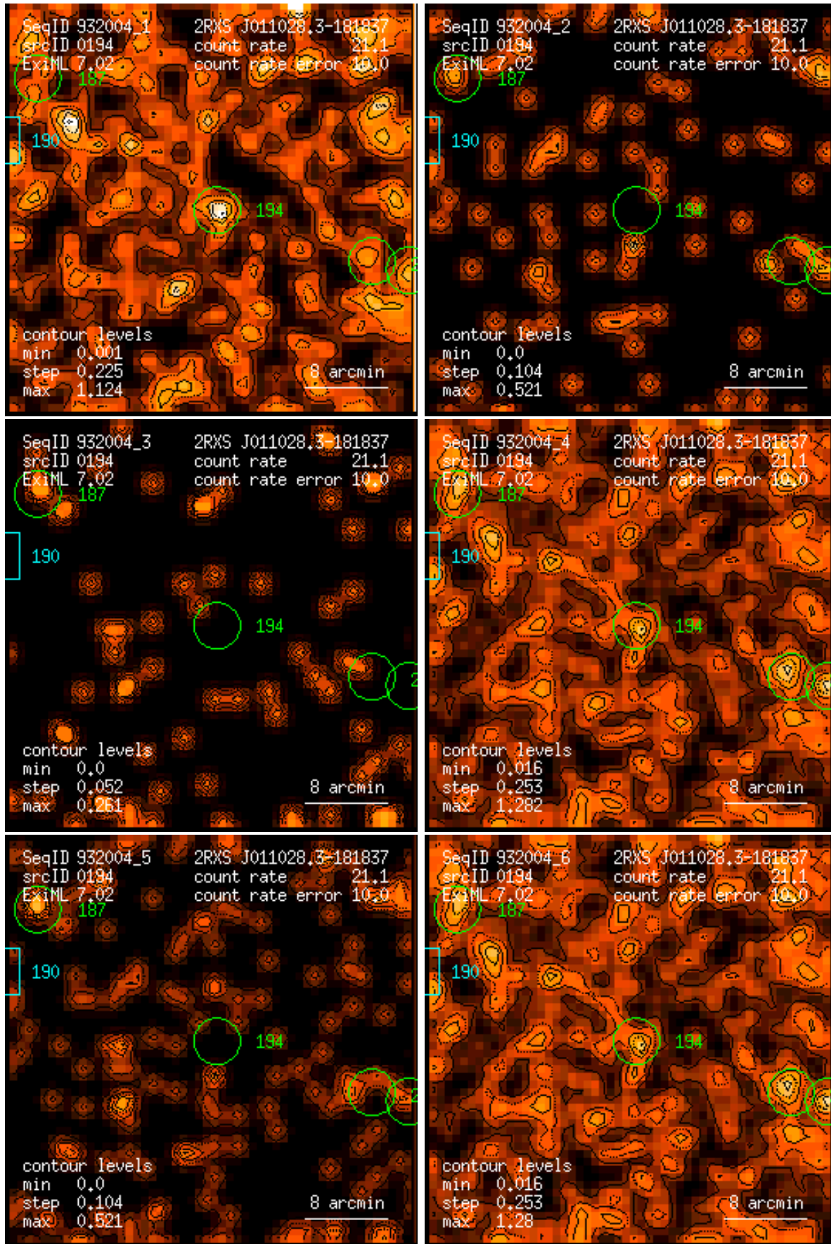
Figure 194: RASS 932004: detection 0194: band rate images, Gaussian filter: (1) PSPC channels 11 – 41, (2) 52 – 90, (3) 91 – 201, (4) 11 – 235, (5) 52 – 201, (6) 11 – 201. Broad band rates in counts/ks. Band rate contour levels in counts/ks/arcmin 2 .
