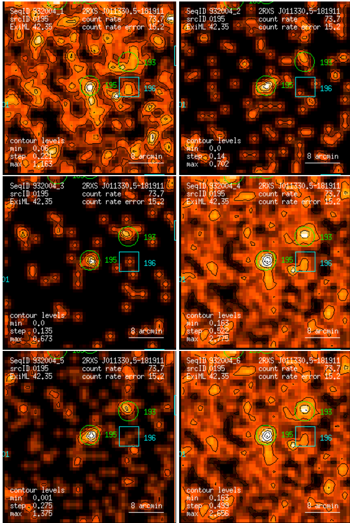
Figure 195: RASS 932004: detection 0195: band rate images, Gaussian filter: (1) PSPC channels 11 – 41, (2) 52 – 90, (3) 91 – 201, (4) 11 – 235, (5) 52 – 201, (6) 11 – 201. Broad band rates in counts/ks. Band rate contour levels in counts/ks/arcmin 2 .
