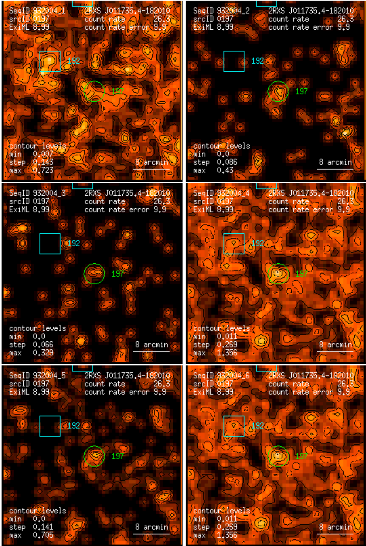
Figure 197: RASS 932004: detection 0197: band rate images, Gaussian filter: (1) PSPC channels 11 – 41, (2) 52 – 90, (3) 91 – 201, (4) 11 – 235, (5) 52 – 201, (6) 11 – 201. Broad band rates in counts/ks. Band rate contour levels in counts/ks/arcmin 2 .
