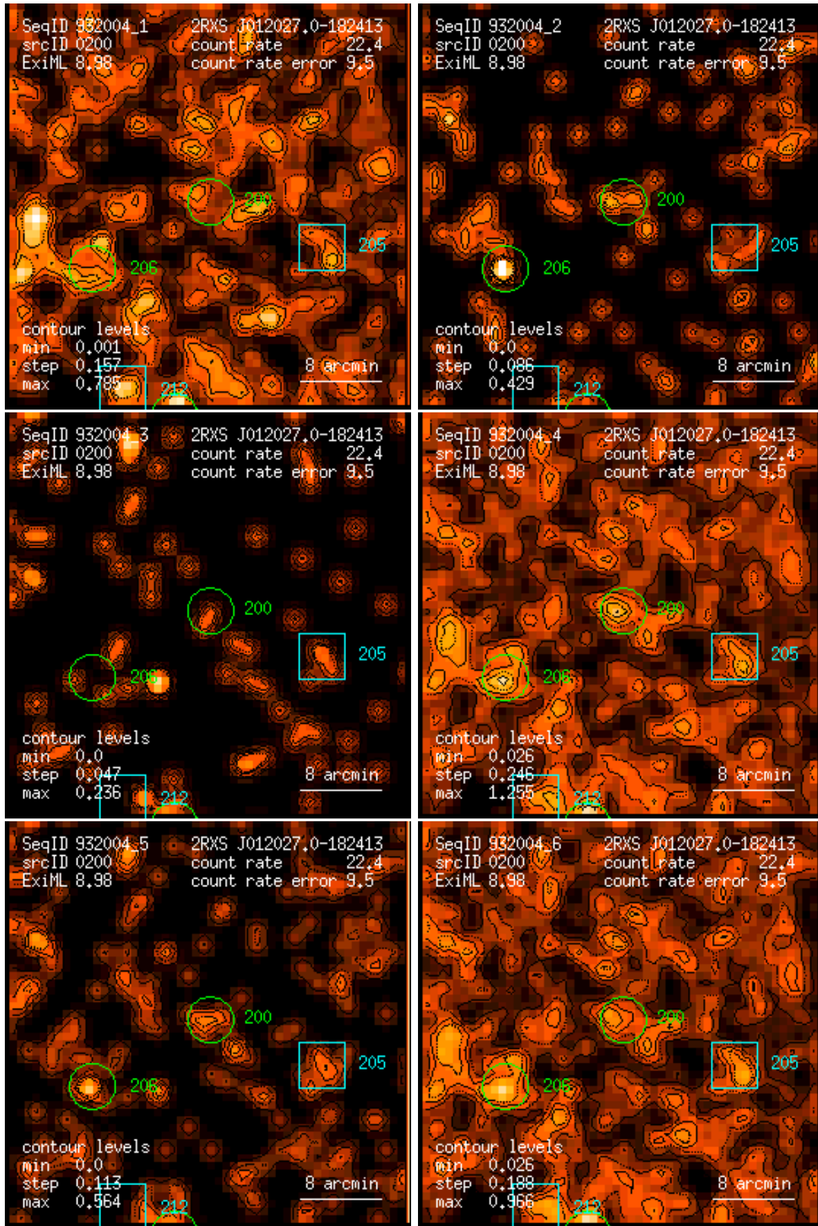
Figure 200: RASS 932004: detection 0200: band rate images, Gaussian filter: (1) PSPC channels 11 – 41, (2) 52 – 90, (3) 91 – 201, (4) 11 – 235, (5) 52 – 201, (6) 11 – 201. Broad band rates in counts/ks. Band rate contour levels in counts/ks/arcmin 2 .
