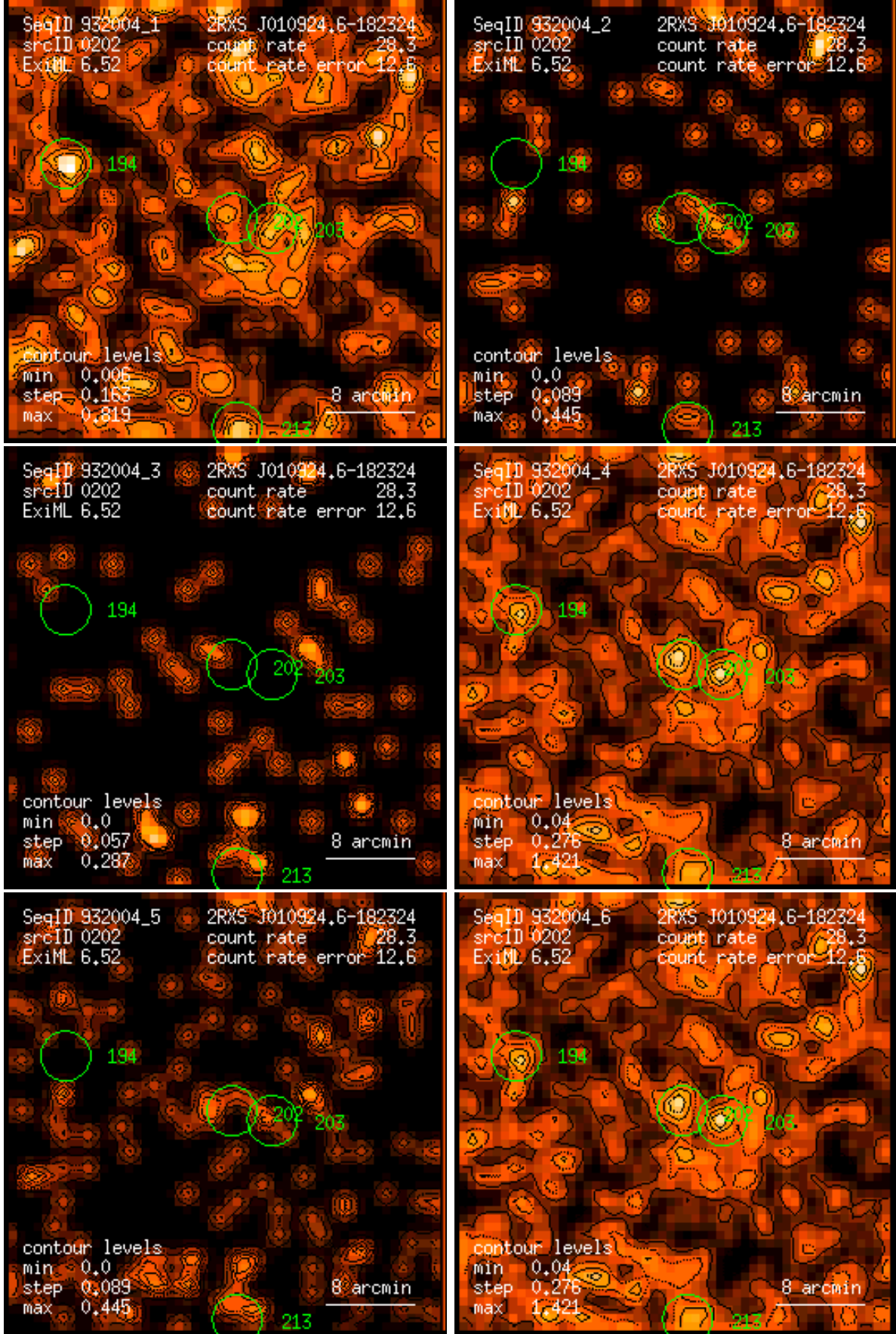
Figure 202: RASS 932004: detection 0202: band rate images, Gaussian filter: (1) PSPC channels 11 – 41, (2) 52 – 90, (3) 91 – 201, (4) 11 – 235, (5) 52 – 201, (6) 11 – 201. Broad band rates in counts/ks. Band rate contour levels in counts/ks/arcmin 2 .
