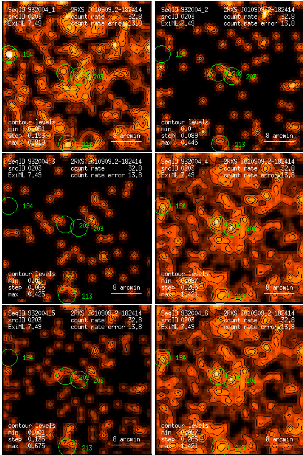
Figure 203: RASS 932004: detection 0203: band rate images, Gaussian filter: (1) PSPC channels 11 – 41, (2) 52 – 90, (3) 91 – 201, (4) 11 – 235, (5) 52 – 201, (6) 11 – 201. Broad band rates in counts/ks. Band rate contour levels in counts/ks/arcmin 2 .
