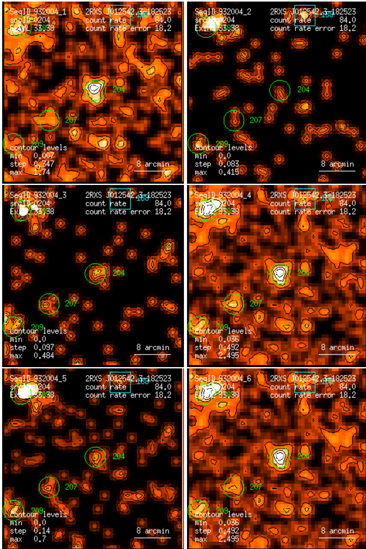
Figure 204: RASS 932004: detection 0204: band rate images, Gaussian filter: (1) PSPC channels 11 – 41, (2) 52 – 90, (3) 91 – 201, (4) 11 – 235, (5) 52 – 201, (6) 11 – 201. Broad band rates in counts/ks. Band rate contour levels in counts/ks/arcmin 2 .
