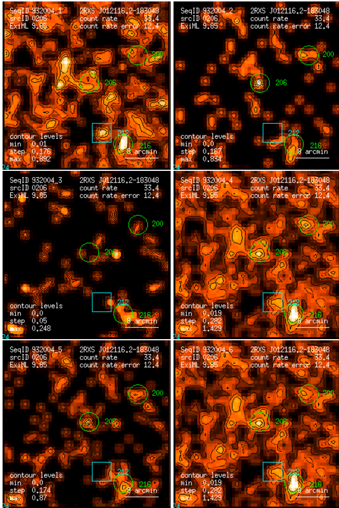
Figure 206: RASS 932004: detection 0206: band rate images, Gaussian filter: (1) PSPC channels 11 – 41, (2) 52 – 90, (3) 91 – 201, (4) 11 – 235, (5) 52 – 201, (6) 11 – 201. Broad band rates in counts/ks. Band rate contour levels in counts/ks/arcmin 2 .
