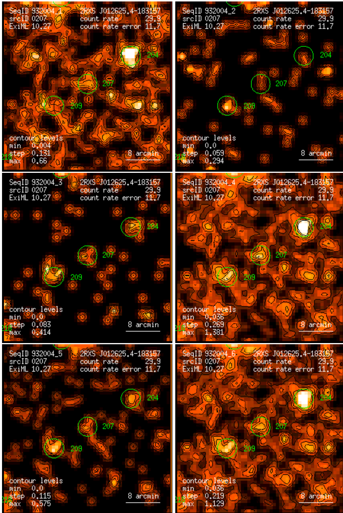
Figure 207: RASS 932004: detection 0207: band rate images, Gaussian filter: (1) PSPC channels 11 – 41, (2) 52 – 90, (3) 91 – 201, (4) 11 – 235, (5) 52 – 201, (6) 11 – 201. Broad band rates in counts/ks. Band rate contour levels in counts/ks/arcmin 2 .
