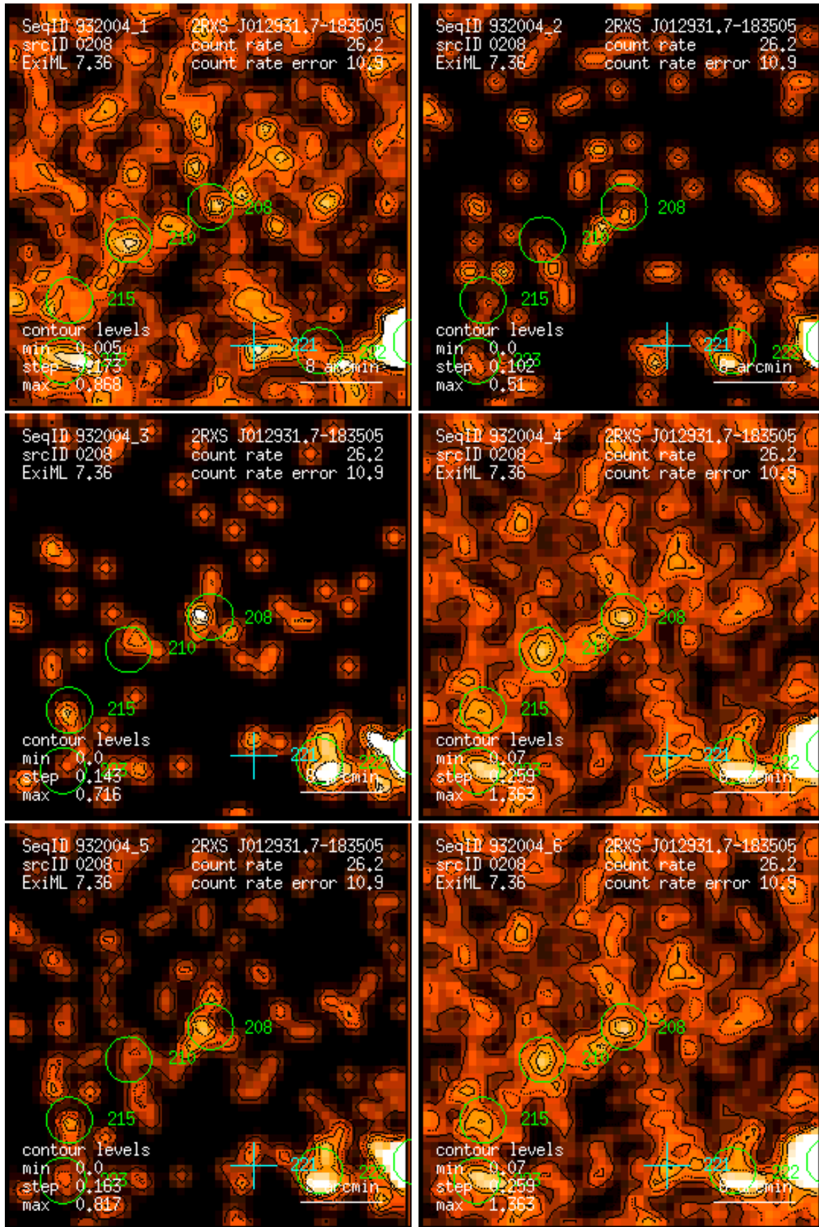
Figure 208: RASS 932004: detection 0208: band rate images, Gaussian filter: (1) PSPC channels 11 – 41, (2) 52 – 90, (3) 91 – 201, (4) 11 – 235, (5) 52 – 201, (6) 11 – 201. Broad band rates in counts/ks. Band rate contour levels in counts/ks/arcmin 2 .
