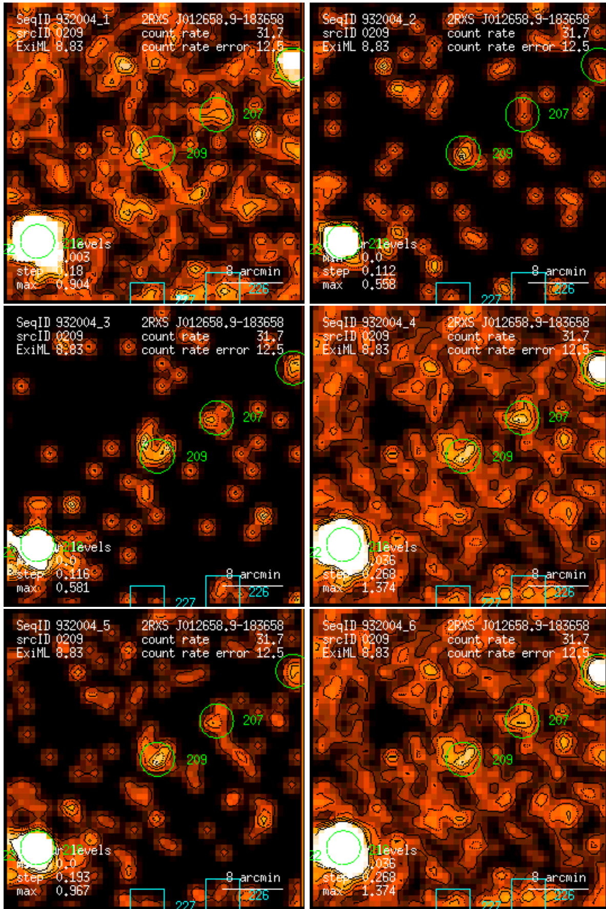
Figure 209: RASS 932004: detection 0209: band rate images, Gaussian filter: (1) PSPC channels 11 – 41, (2) 52 – 90, (3) 91 – 201, (4) 11 – 235, (5) 52 – 201, (6) 11 – 201. Broad band rates in counts/ks. Band rate contour levels in counts/ks/arcmin 2 .
