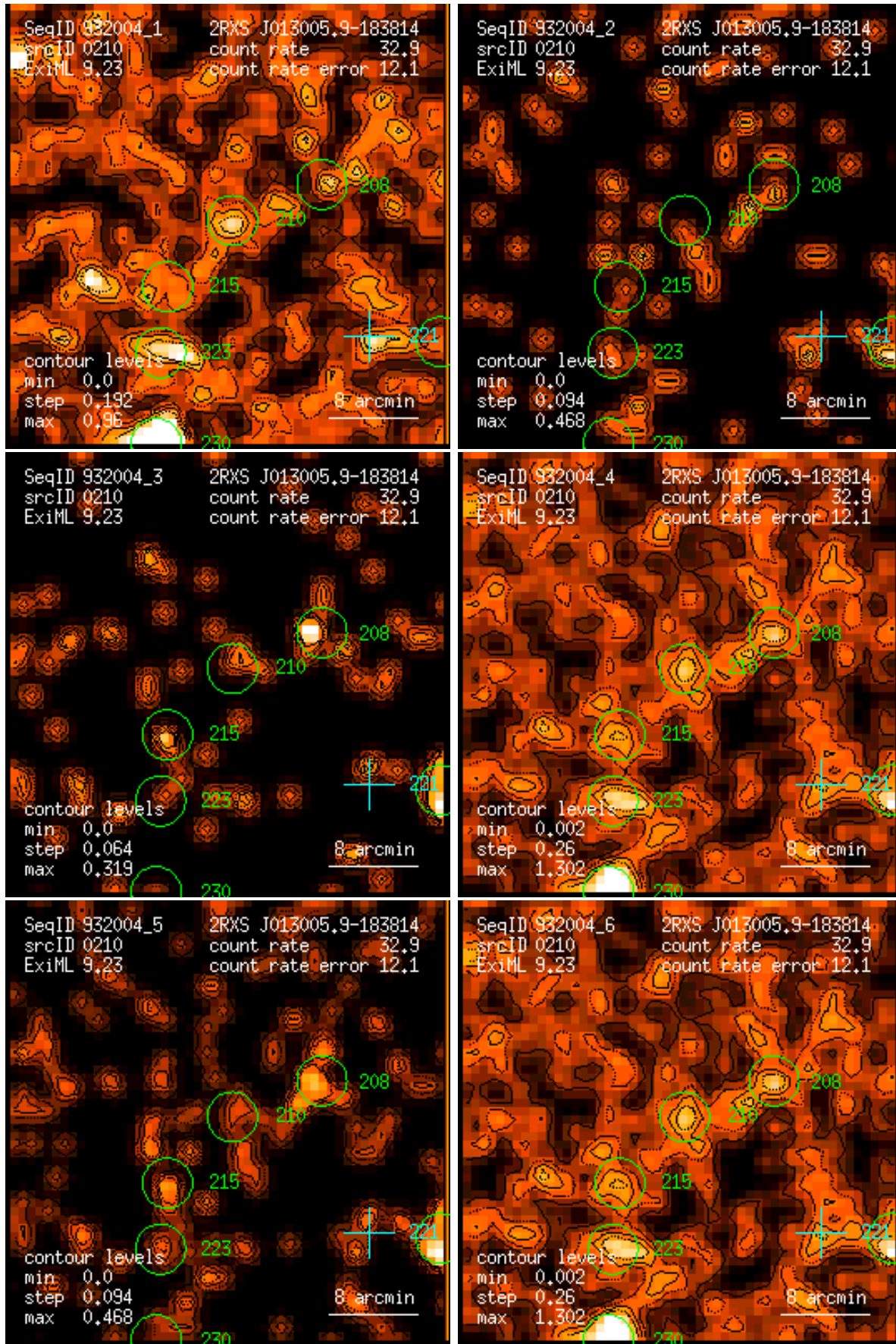
Figure 210: RASS 932004: detection 0210: band rate images, Gaussian filter: (1) PSPC channels 11 – 41, (2) 52 – 90, (3) 91 – 201, (4) 11 – 235, (5) 52 – 201, (6) 11 – 201. Broad band rates in counts/ks. Band rate contour levels in counts/ks/arcmin 2 .
