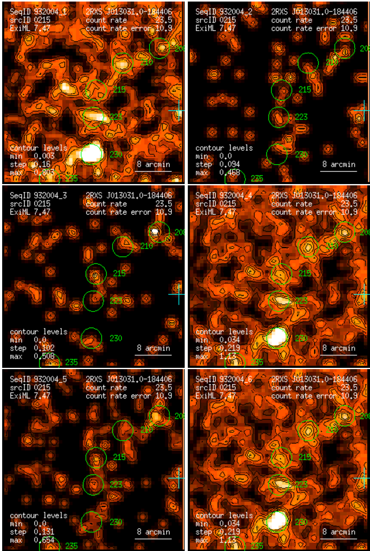
Figure 215: RASS 932004: detection 0215: band rate images, Gaussian filter: (1) PSPC channels 11 – 41, (2) 52 – 90, (3) 91 – 201, (4) 11 – 235, (5) 52 – 201, (6) 11 – 201. Broad band rates in counts/ks. Band rate contour levels in counts/ks/arcmin 2 .
