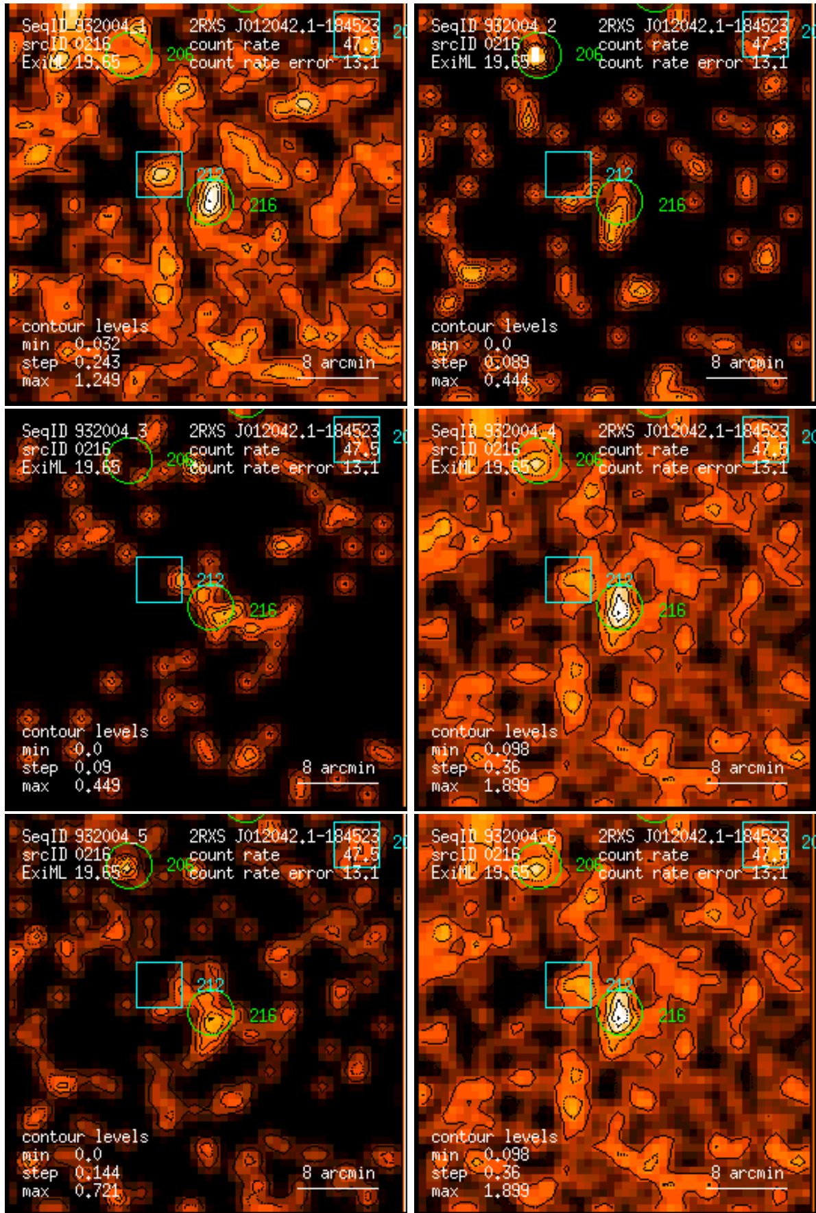
Figure 216: RASS 932004: detection 0216: band rate images, Gaussian filter: (1) PSPC channels 11 – 41, (2) 52 – 90, (3) 91 – 201, (4) 11 – 235, (5) 52 – 201, (6) 11 – 201. Broad band rates in counts/ks. Band rate contour levels in counts/ks/arcmin 2 .
