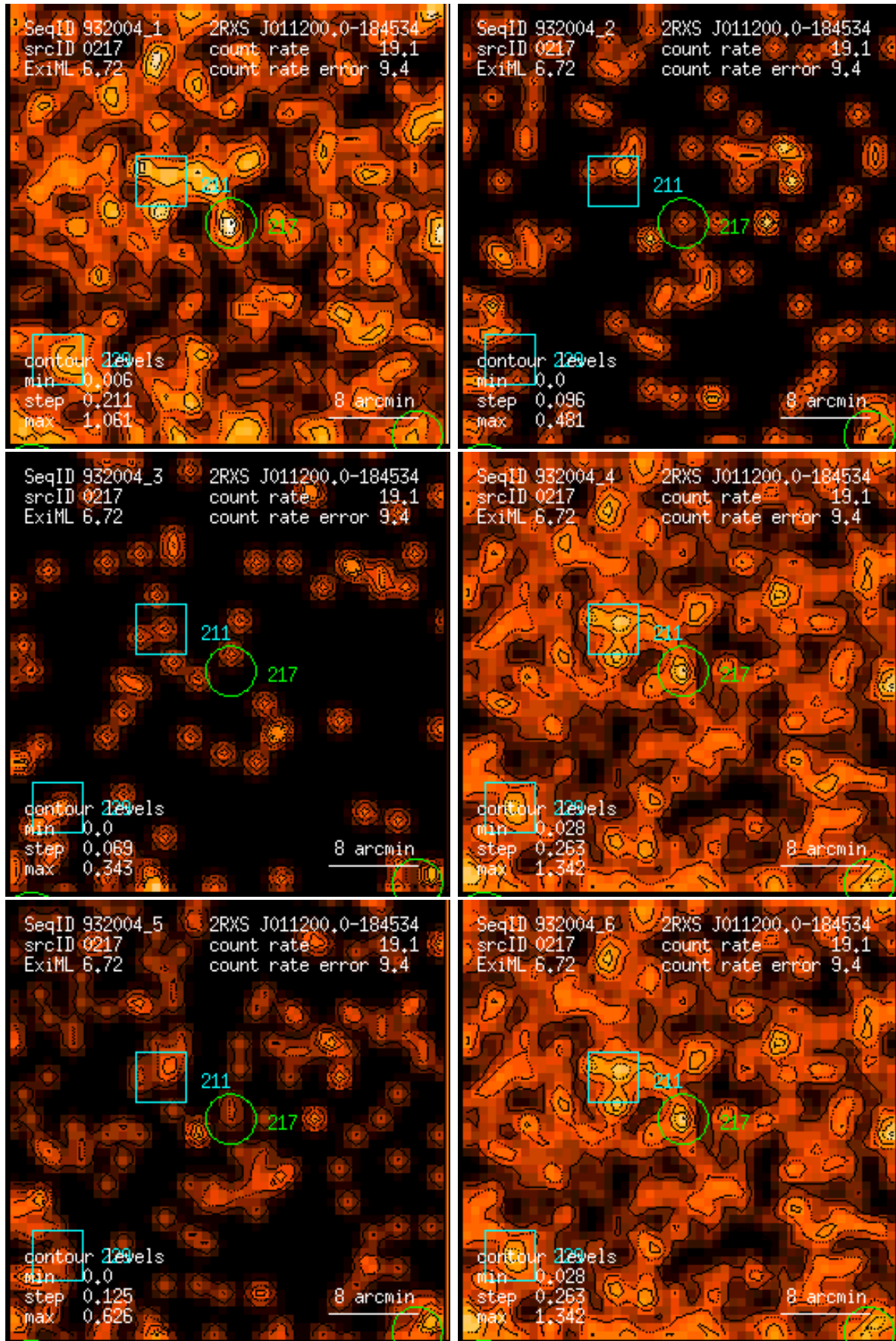
Figure 217: RASS 932004: detection 0217: band rate images, Gaussian filter: (1) PSPC channels 11 – 41, (2) 52 – 90, (3) 91 – 201, (4) 11 – 235, (5) 52 – 201, (6) 11 – 201. Broad band rates in counts/ks. Band rate contour levels in counts/ks/arcmin 2 .
