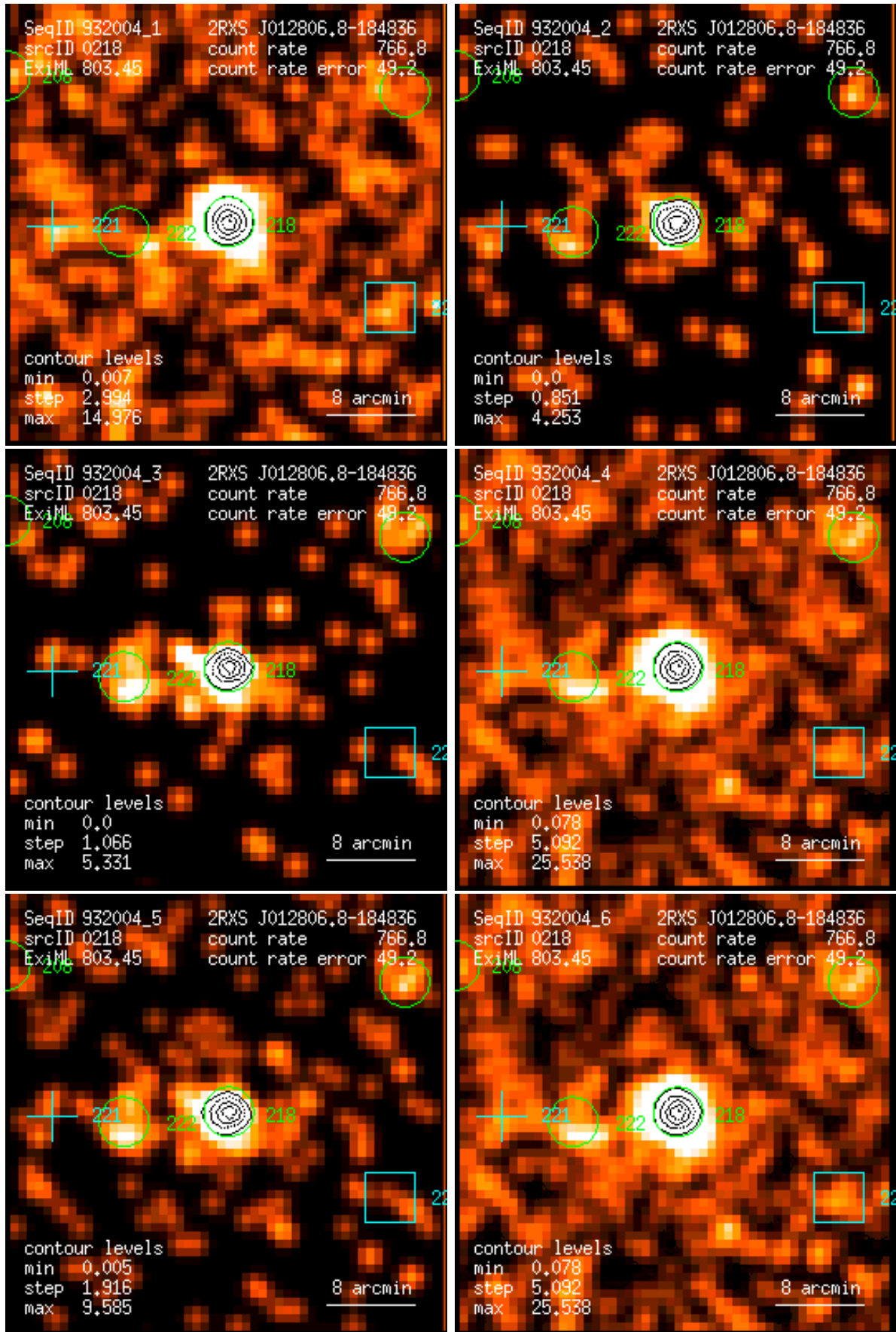
Figure 218: RASS 932004: detection 0218: band rate images, Gaussian filter: (1) PSPC channels 11 – 41, (2) 52 – 90, (3) 91 – 201, (4) 11 – 235, (5) 52 – 201, (6) 11 – 201. Broad band rates in counts/ks. Band rate contour levels in counts/ks/arcmin 2 .
