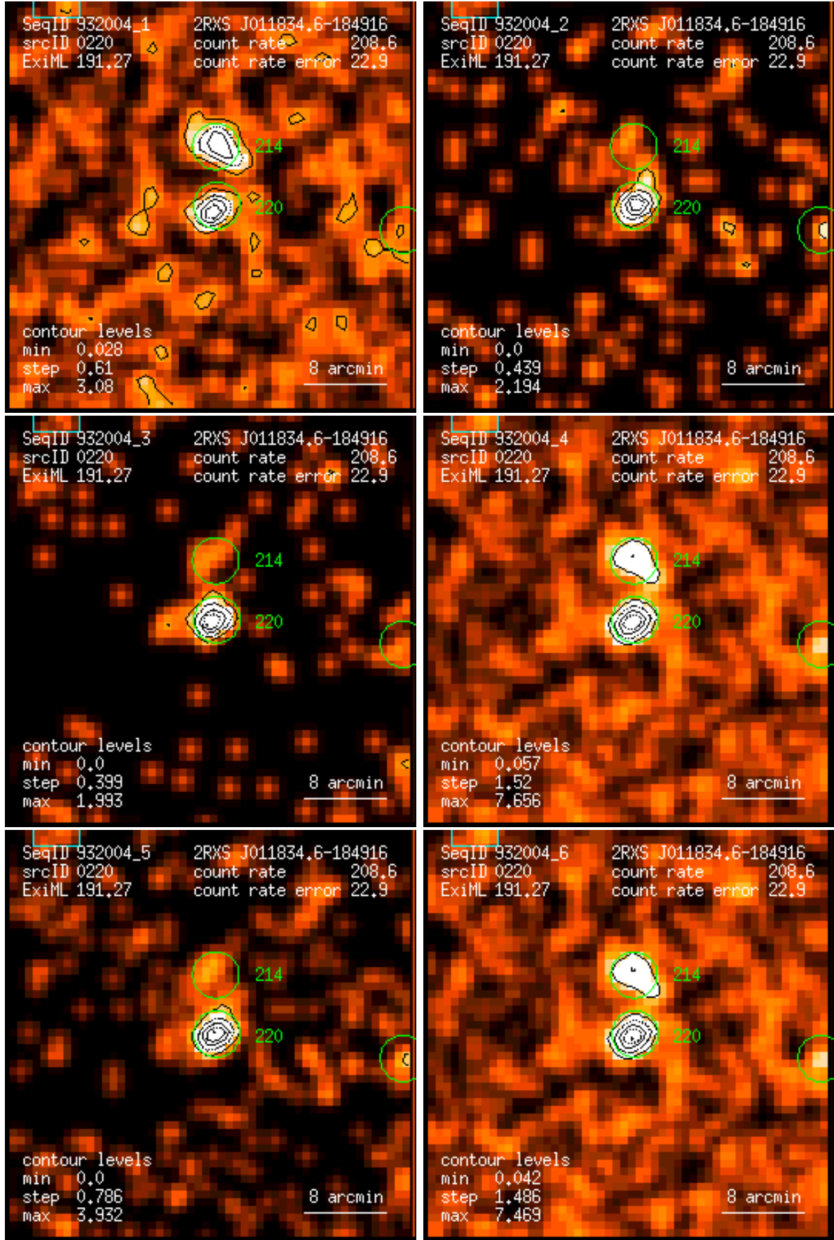
Figure 220: RASS 932004: detection 0220: band rate images, Gaussian filter: (1) PSPC channels 11 – 41, (2) 52 – 90, (3) 91 – 201, (4) 11 – 235, (5) 52 – 201, (6) 11 – 201. Broad band rates in counts/ks. Band rate contour levels in counts/ks/arcmin 2 .
