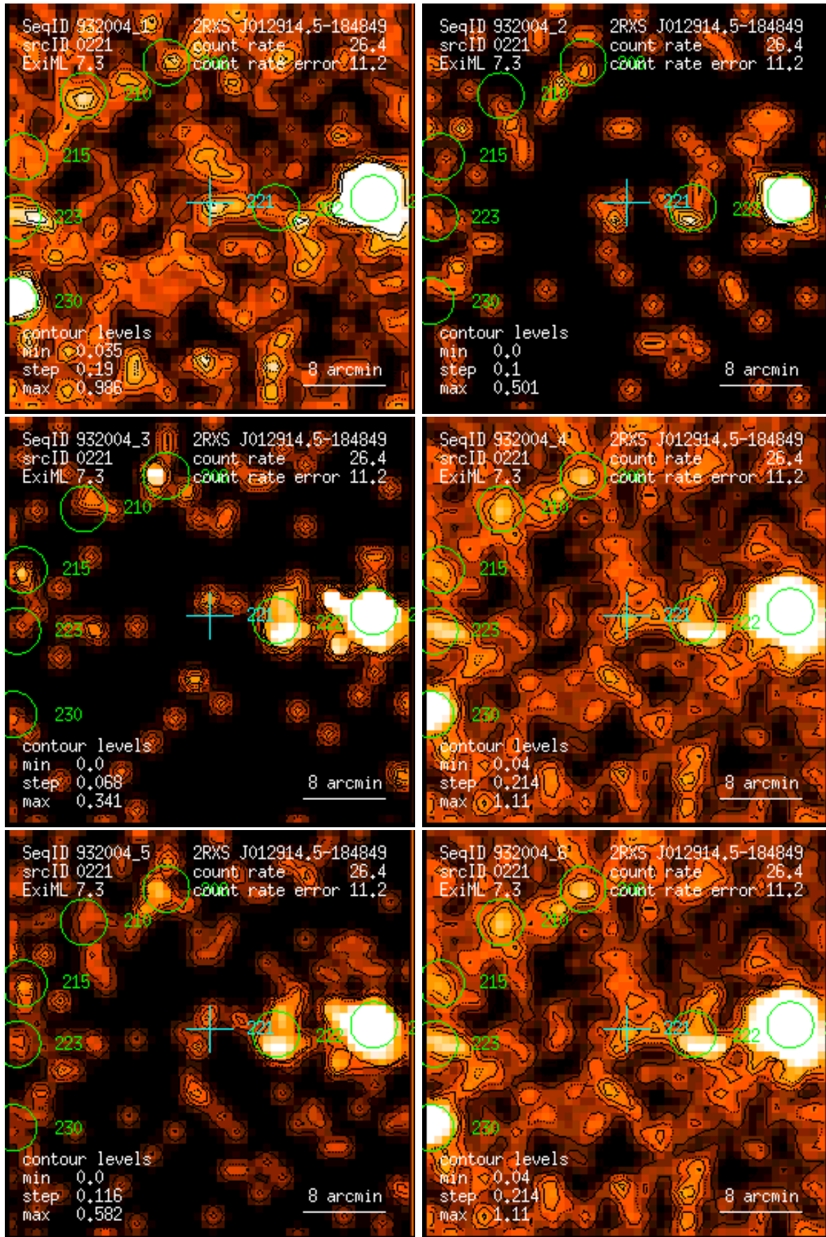
Figure 221: RASS 932004: detection 0221: band rate images, Gaussian filter: (1) PSPC channels 11 – 41, (2) 52 – 90, (3) 91 – 201, (4) 11 – 235, (5) 52 – 201, (6) 11 – 201. Broad band rates in counts/ks. Band rate contour levels in counts/ks/arcmin 2 .
