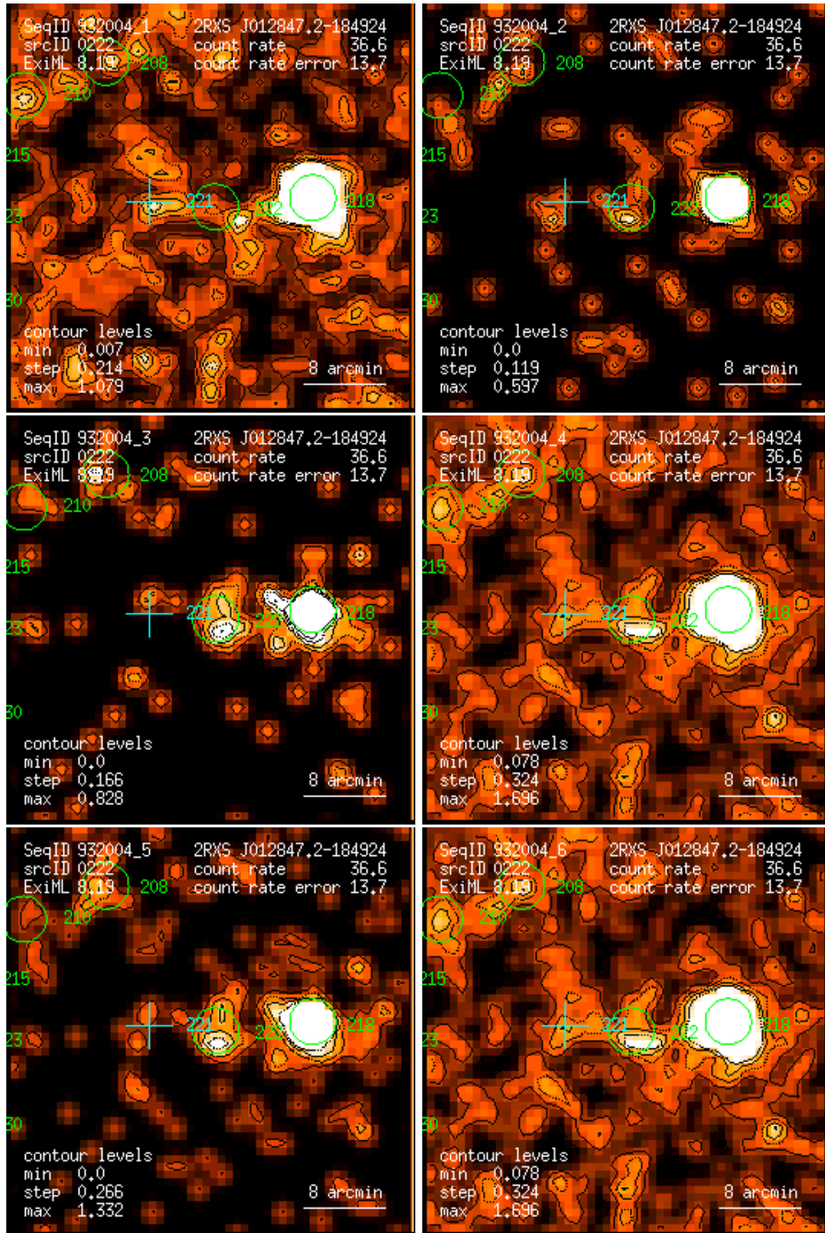
Figure 222: RASS 932004: detection 0222: band rate images, Gaussian filter: (1) PSPC channels 11 – 41, (2) 52 – 90, (3) 91 – 201, (4) 11 – 235, (5) 52 – 201, (6) 11 – 201. Broad band rates in counts/ks. Band rate contour levels in counts/ks/arcmin 2 .
