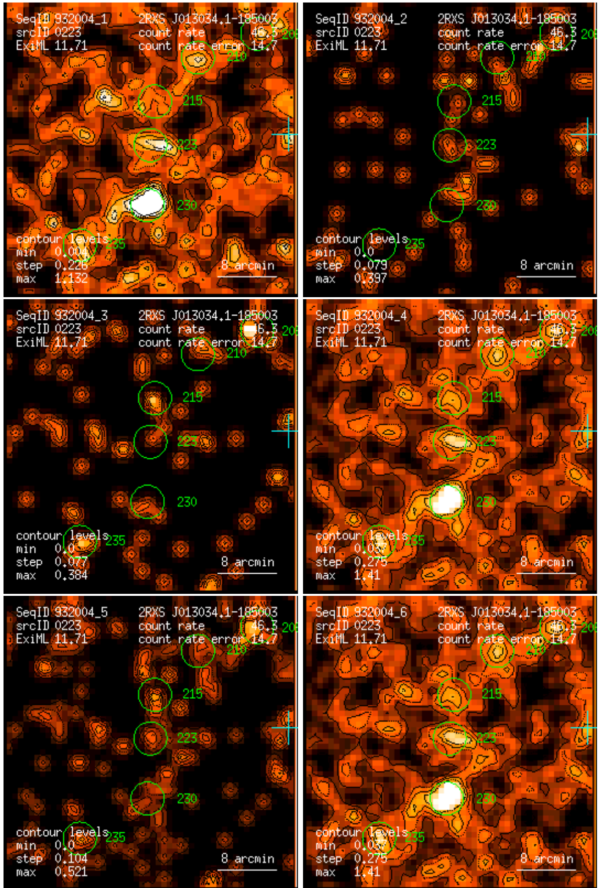
Figure 223: RASS 932004: detection 0223: band rate images, Gaussian filter: (1) PSPC channels 11 – 41, (2) 52 – 90, (3) 91 – 201, (4) 11 – 235, (5) 52 – 201, (6) 11 – 201. Broad band rates in counts/ks. Band rate contour levels in counts/ks/arcmin 2 .
