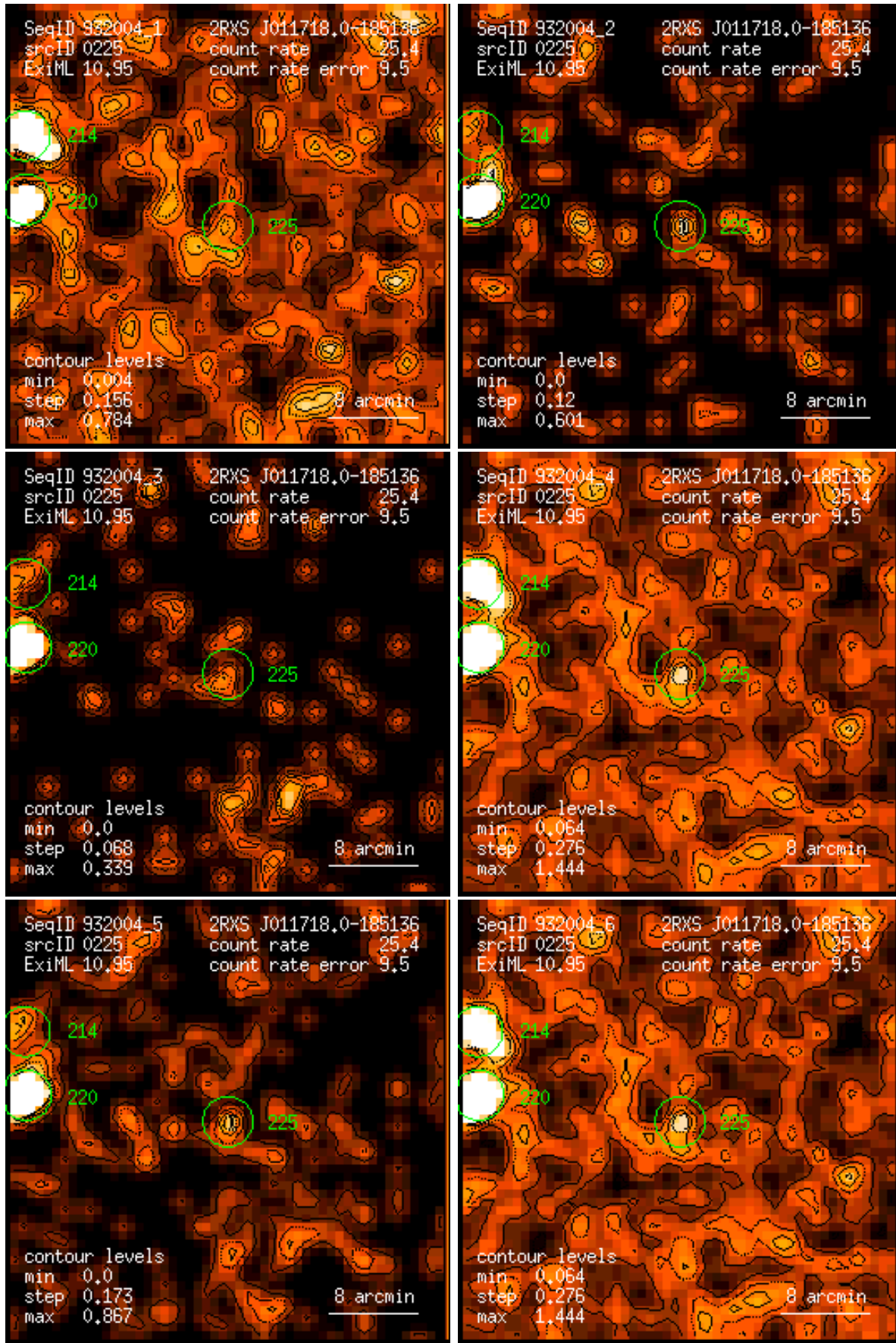
Figure 225: RASS 932004: detection 0225: band rate images, Gaussian filter: (1) PSPC channels 11 – 41, (2) 52 – 90, (3) 91 – 201, (4) 11 – 235, (5) 52 – 201, (6) 11 – 201. Broad band rates in counts/ks. Band rate contour levels in counts/ks/arcmin 2 .
