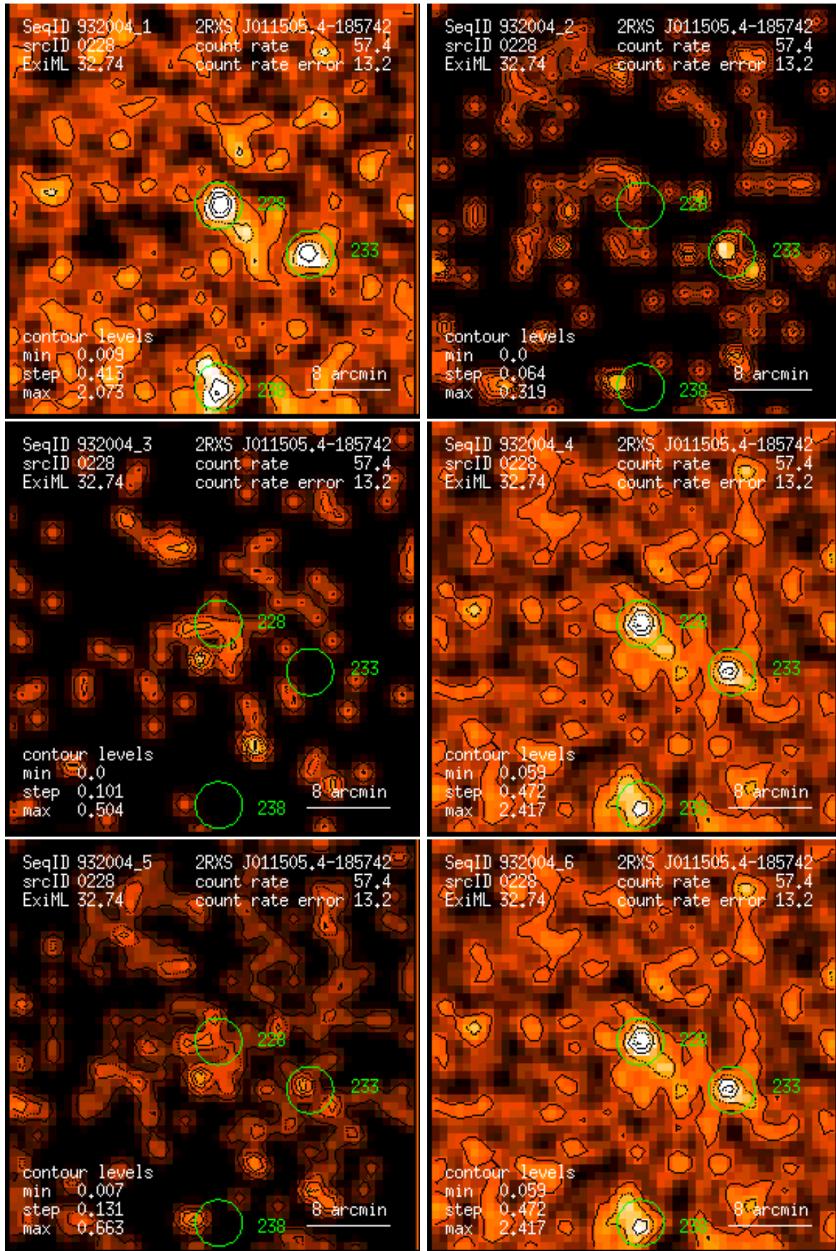
Figure 228: RASS 932004: detection 0228: band rate images, Gaussian filter: (1) PSPC channels 11 – 41, (2) 52 – 90, (3) 91 – 201, (4) 11 – 235, (5) 52 – 201, (6) 11 – 201. Broad band rates in counts/ks. Band rate contour levels in counts/ks/arcmin 2 .
